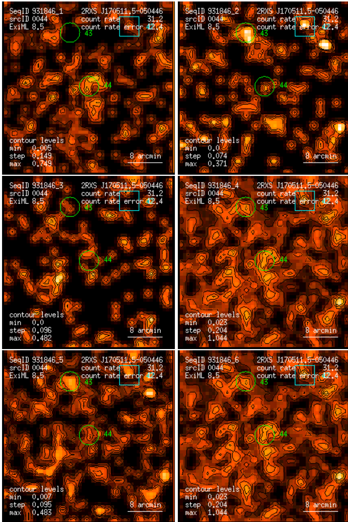
Figure 44: RASS 931846: detection 0044: band rate images, Gaussian filter: (1) PSPC channels 11 – 41, (2) 52 – 90, (3) 91 – 201, (4) 11 – 235, (5) 52 – 201, (6) 11 – 201. Broad band rates in counts/ks. Band rate contour levels in counts/ks/arcmin 2 .
