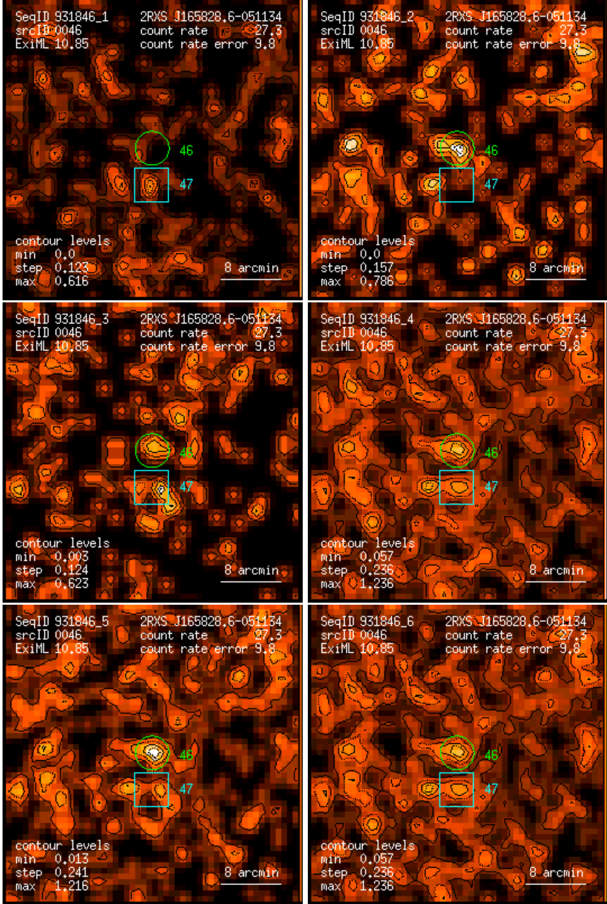
Figure 46: RASS 931846: detection 0046: band rate images, Gaussian filter: (1) PSPC channels 11 – 41, (2) 52 – 90, (3) 91 – 201, (4) 11 – 235, (5) 52 – 201, (6) 11 – 201. Broad band rates in counts/ks. Band rate contour levels in counts/ks/arcmin 2 .
