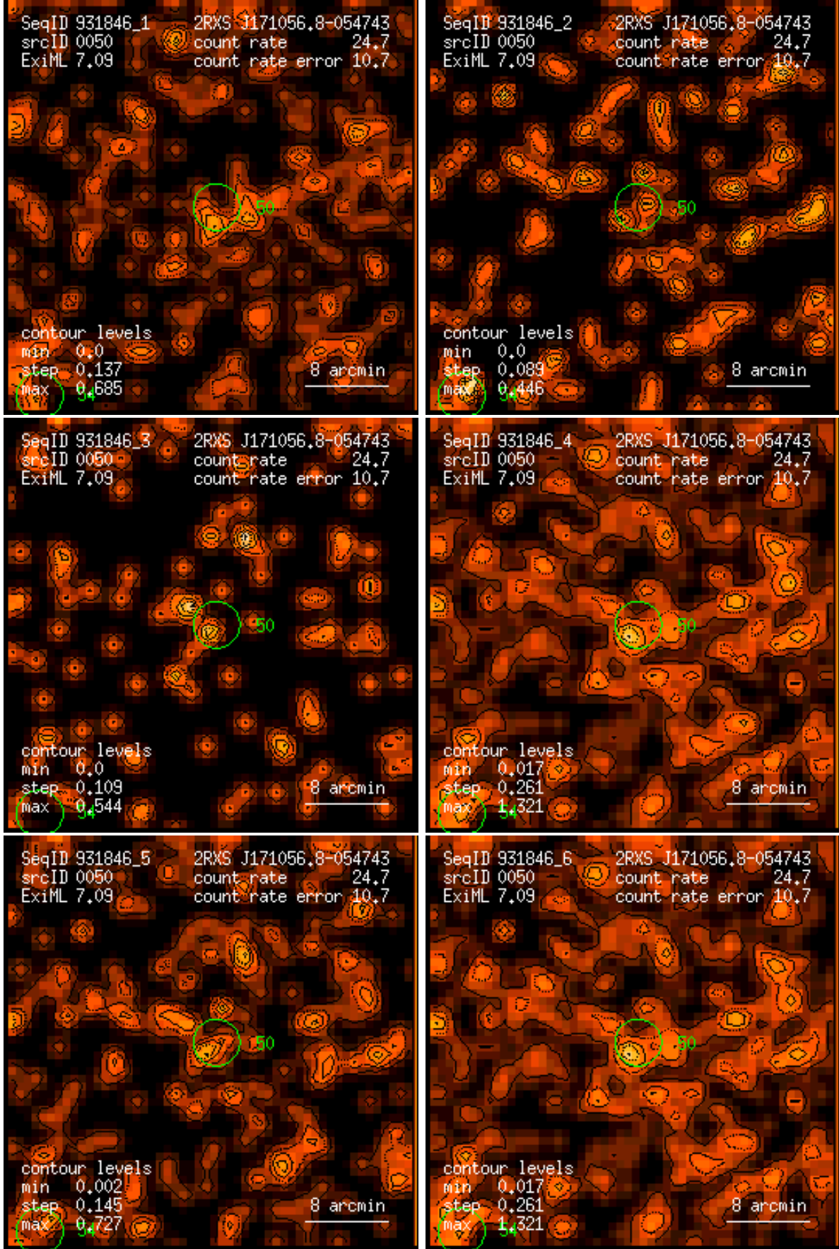
Figure 50: RASS 931846: detection 0050: band rate images, Gaussian filter: (1) PSPC channels 11 – 41, (2) 52 – 90, (3) 91 – 201, (4) 11 – 235, (5) 52 – 201, (6) 11 – 201. Broad band rates in counts/ks. Band rate contour levels in counts/ks/arcmin 2 .
