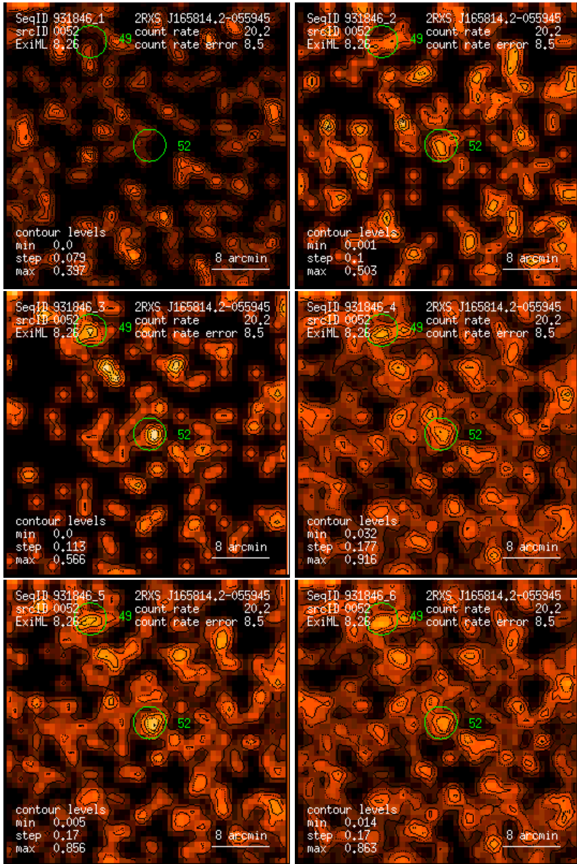
Figure 52: RASS 931846: detection 0052: band rate images, Gaussian filter: (1) PSPC channels 11 – 41, (2) 52 – 90, (3) 91 – 201, (4) 11 – 235, (5) 52 – 201, (6) 11 – 201. Broad band rates in counts/ks. Band rate contour levels in counts/ks/arcmin 2 .
