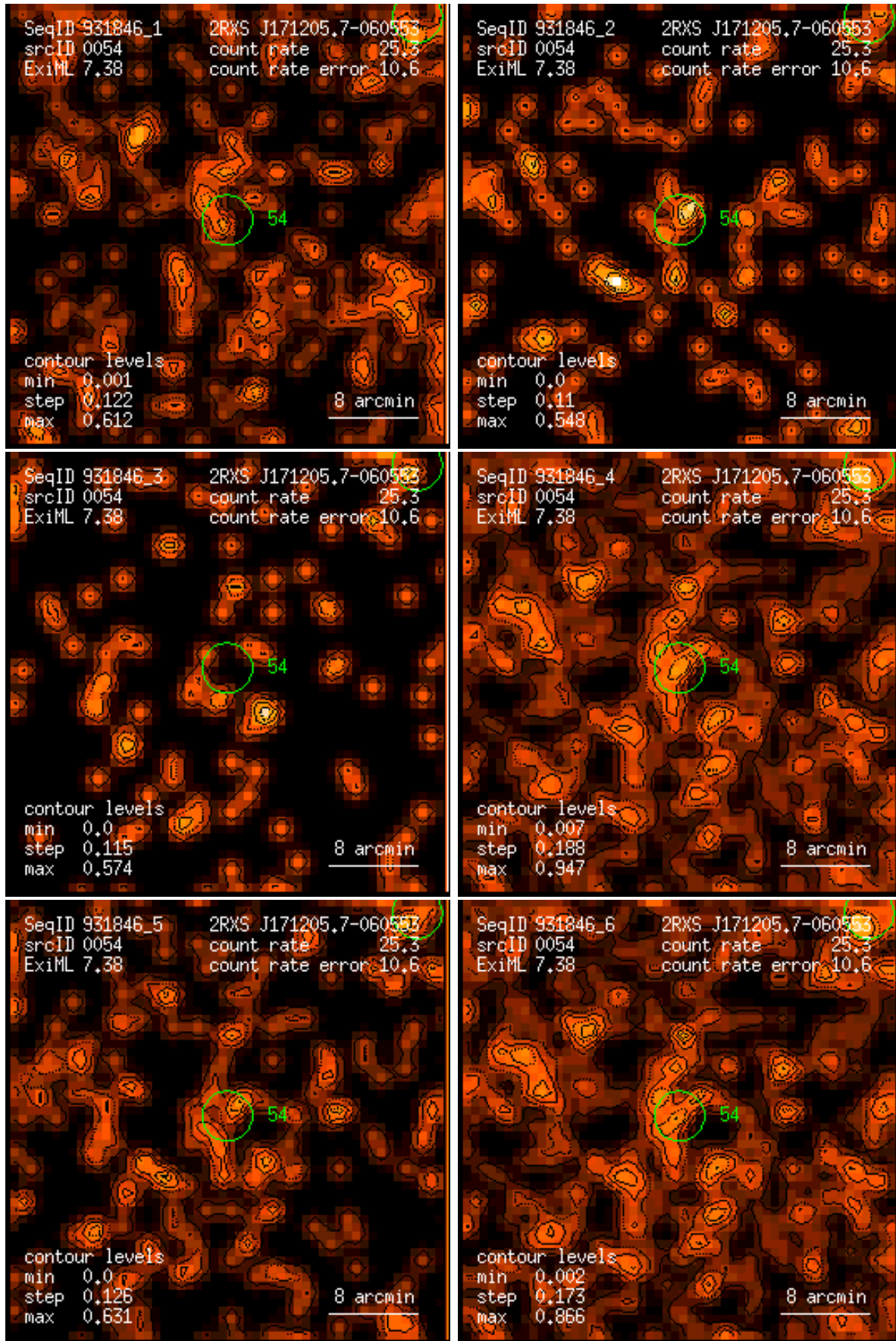
Figure 54: RASS 931846: detection 0054: band rate images, Gaussian filter: (1) PSPC channels 11 – 41, (2) 52 – 90, (3) 91 – 201, (4) 11 – 235, (5) 52 – 201, (6) 11 – 201. Broad band rates in counts/ks. Band rate contour levels in counts/ks/arcmin 2 .
