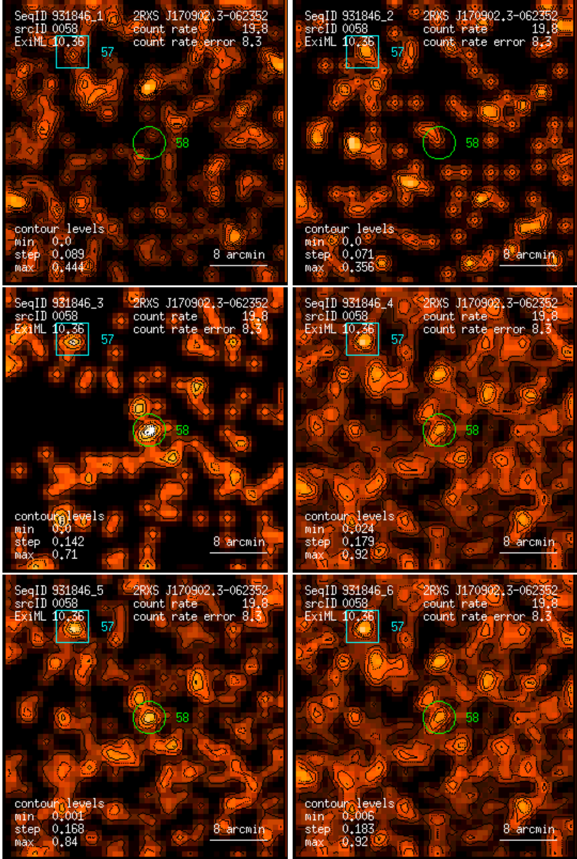
Figure 58: RASS 931846: detection 0058: band rate images, Gaussian filter: (1) PSPC channels 11 – 41, (2) 52 – 90, (3) 91 – 201, (4) 11 – 235, (5) 52 – 201, (6) 11 – 201. Broad band rates in counts/ks. Band rate contour levels in counts/ks/arcmin 2 .
