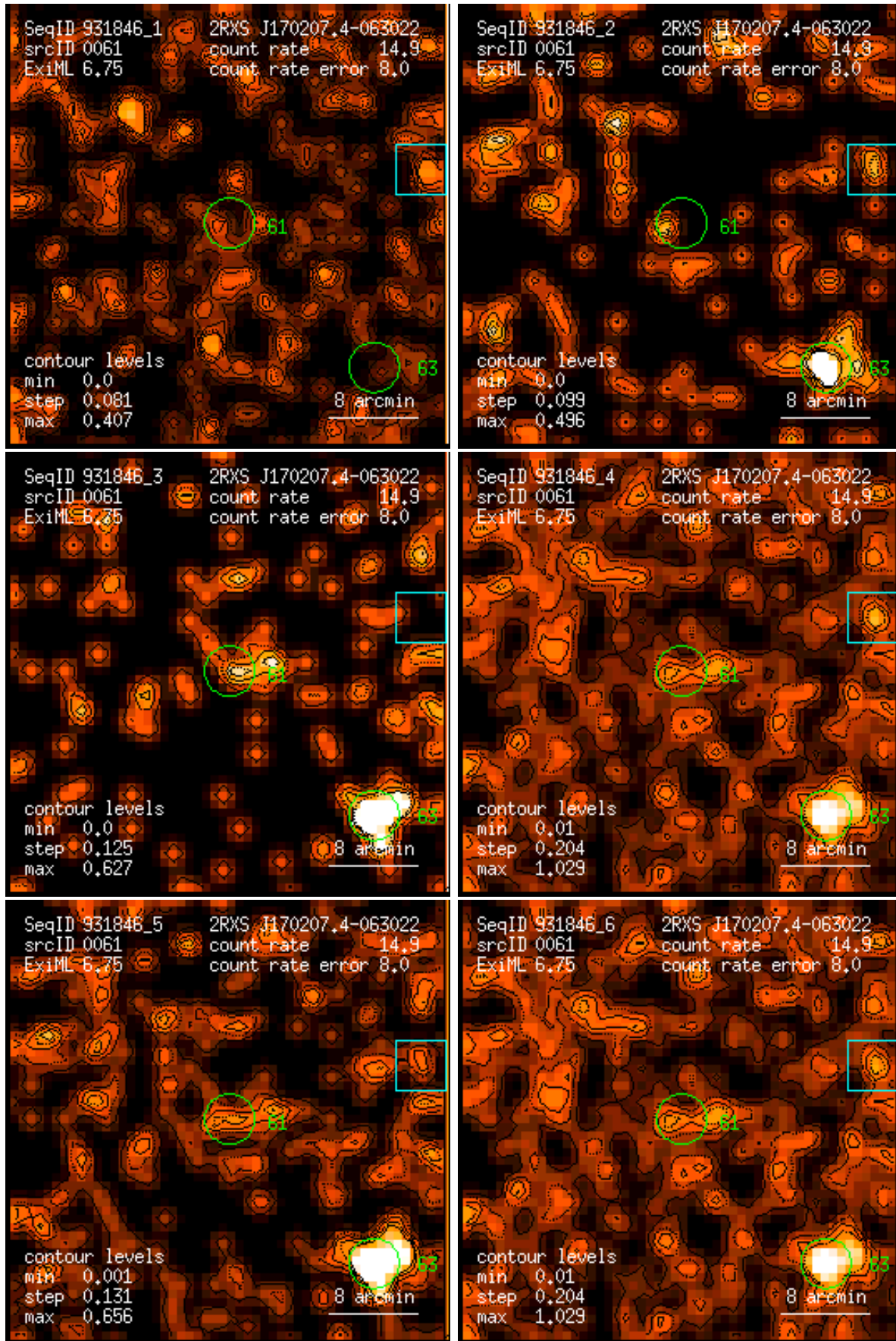
Figure 61: RASS 931846: detection 0061: band rate images, Gaussian filter: (1) PSPC channels 11 – 41, (2) 52 – 90, (3) 91 – 201, (4) 11 – 235, (5) 52 – 201, (6) 11 – 201. Broad band rates in counts/ks. Band rate contour levels in counts/ks/arcmin 2 .
