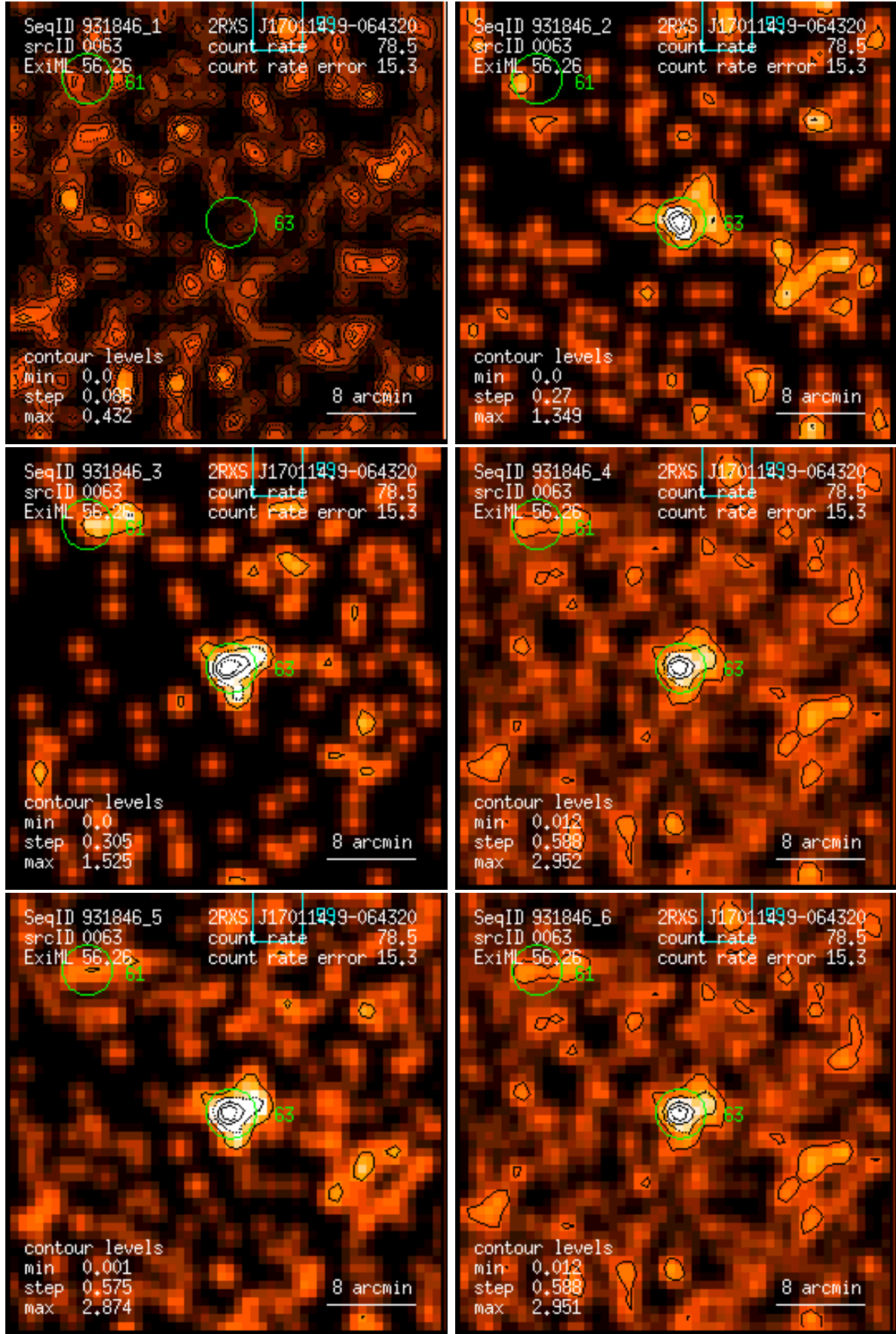
Figure 63: RASS 931846: detection 0063: band rate images, Gaussian filter: (1) PSPC channels 11 – 41, (2) 52 – 90, (3) 91 – 201, (4) 11 – 235, (5) 52 – 201, (6) 11 – 201. Broad band rates in counts/ks. Band rate contour levels in counts/ks/arcmin 2 .
