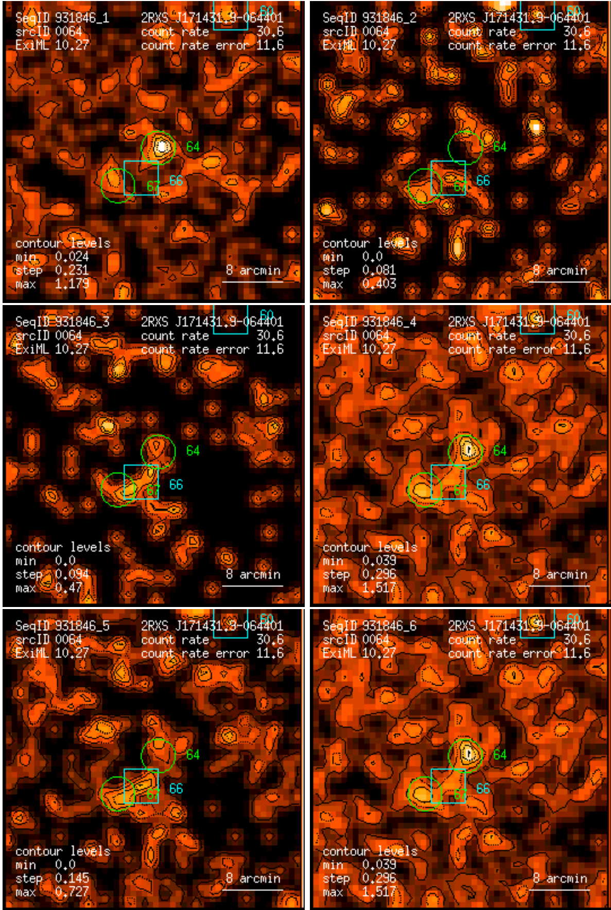
Figure 64: RASS 931846: detection 0064: band rate images, Gaussian filter: (1) PSPC channels 11 – 41, (2) 52 – 90, (3) 91 – 201, (4) 11 – 235, (5) 52 – 201, (6) 11 – 201. Broad band rates in counts/ks. Band rate contour levels in counts/ks/arcmin 2 .
