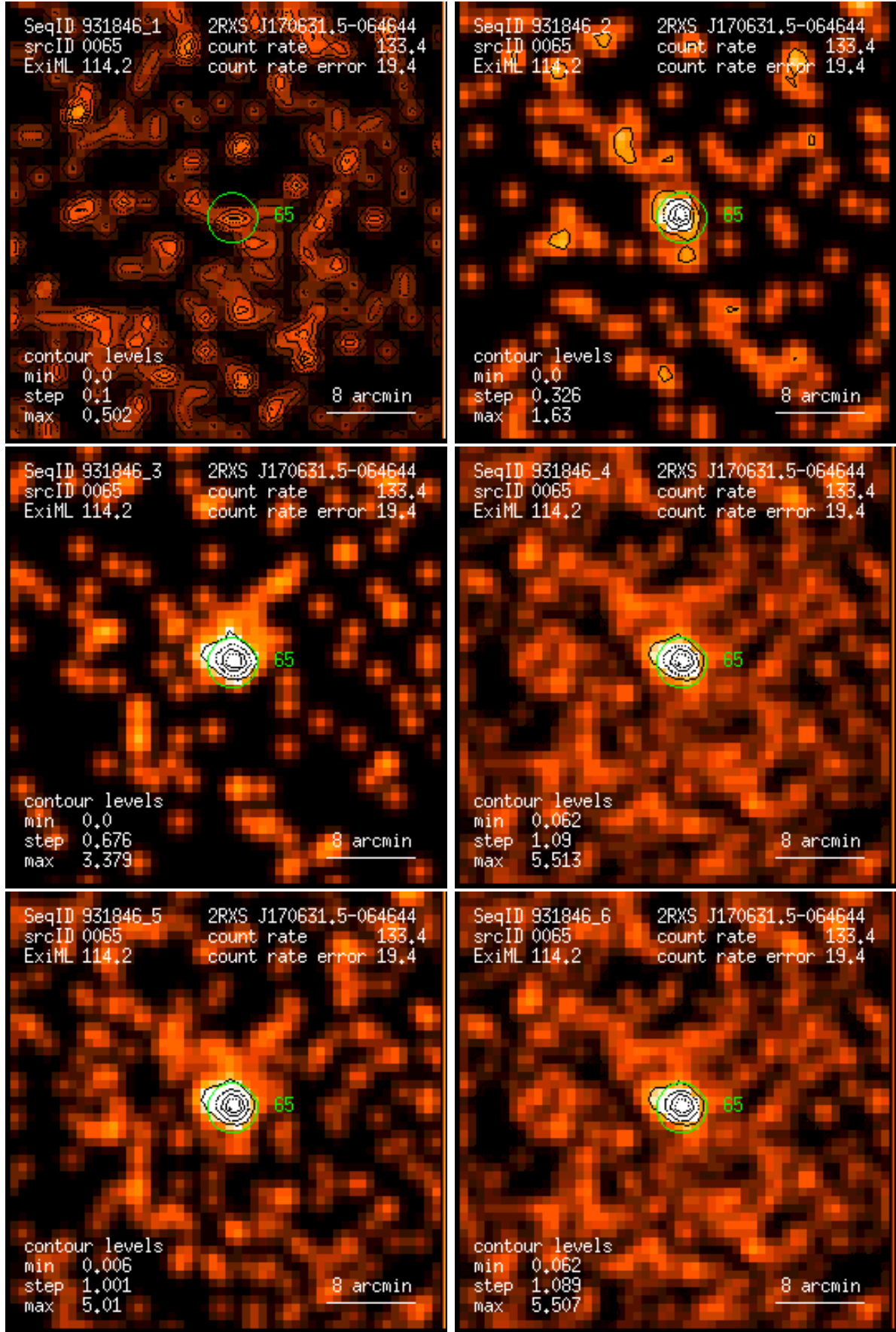
Figure 65: RASS 931846: detection 0065: band rate images, Gaussian filter: (1) PSPC channels 11 – 41, (2) 52 – 90, (3) 91 – 201, (4) 11 – 235, (5) 52 – 201, (6) 11 – 201. Broad band rates in counts/ks. Band rate contour levels in counts/ks/arcmin 2 .
