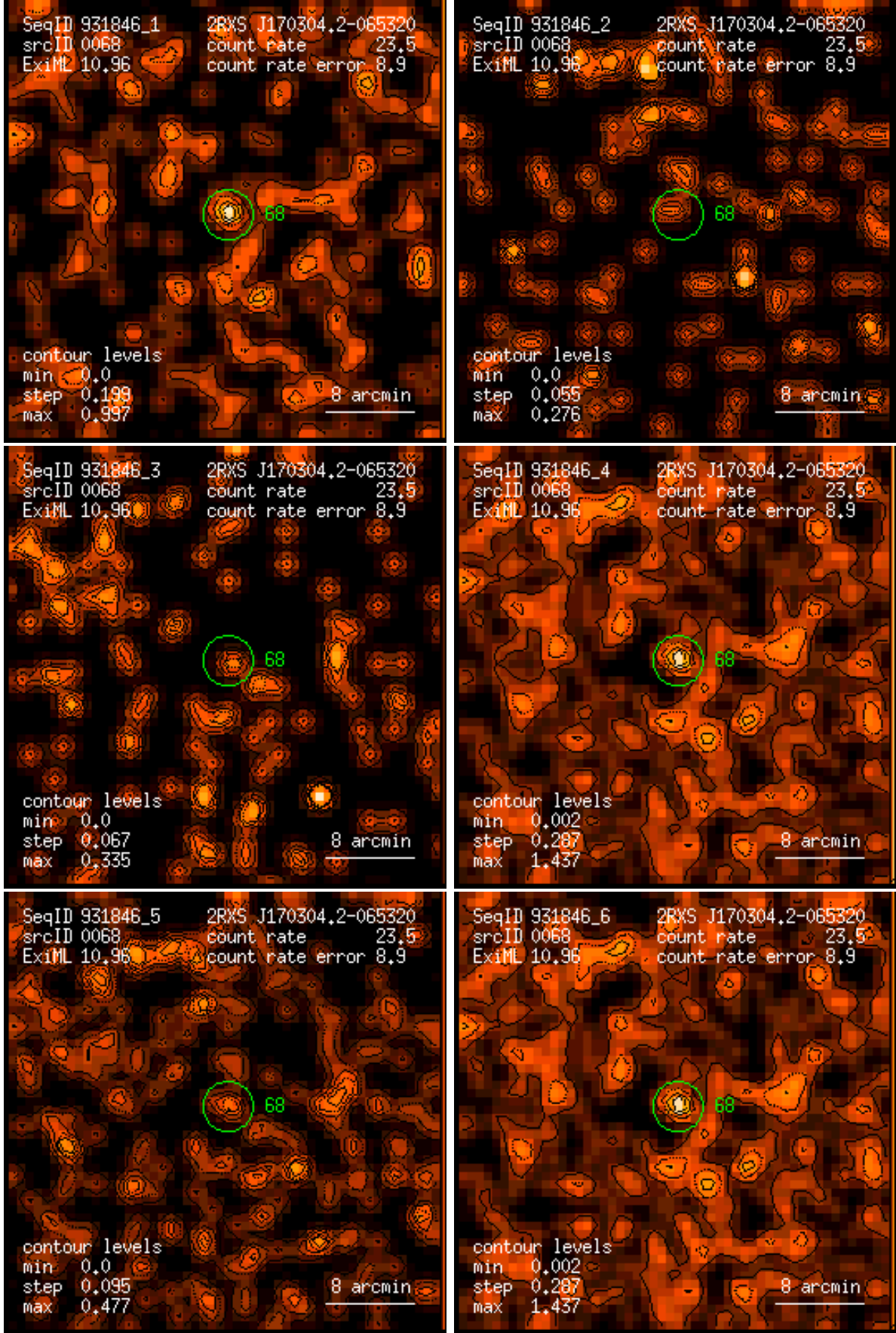
Figure 68: RASS 931846: detection 0068: band rate images, Gaussian filter: (1) PSPC channels 11 – 41, (2) 52 – 90, (3) 91 – 201, (4) 11 – 235, (5) 52 – 201, (6) 11 – 201. Broad band rates in counts/ks. Band rate contour levels in counts/ks/arcmin 2 .
