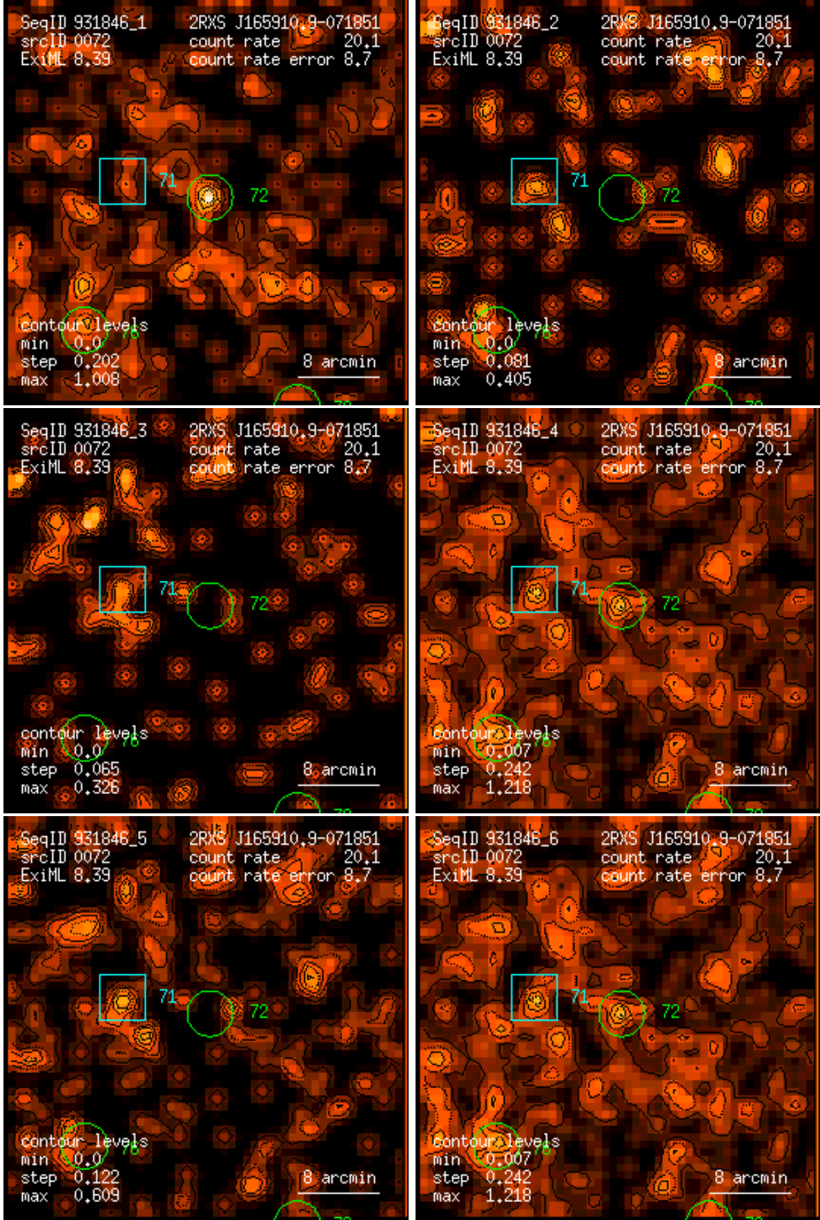
Figure 72: RASS 931846: detection 0072: band rate images, Gaussian filter: (1) PSPC channels 11 – 41, (2) 52 – 90, (3) 91 – 201, (4) 11 – 235, (5) 52 – 201, (6) 11 – 201. Broad band rates in counts/ks. Band rate contour levels in counts/ks/arcmin 2 .
