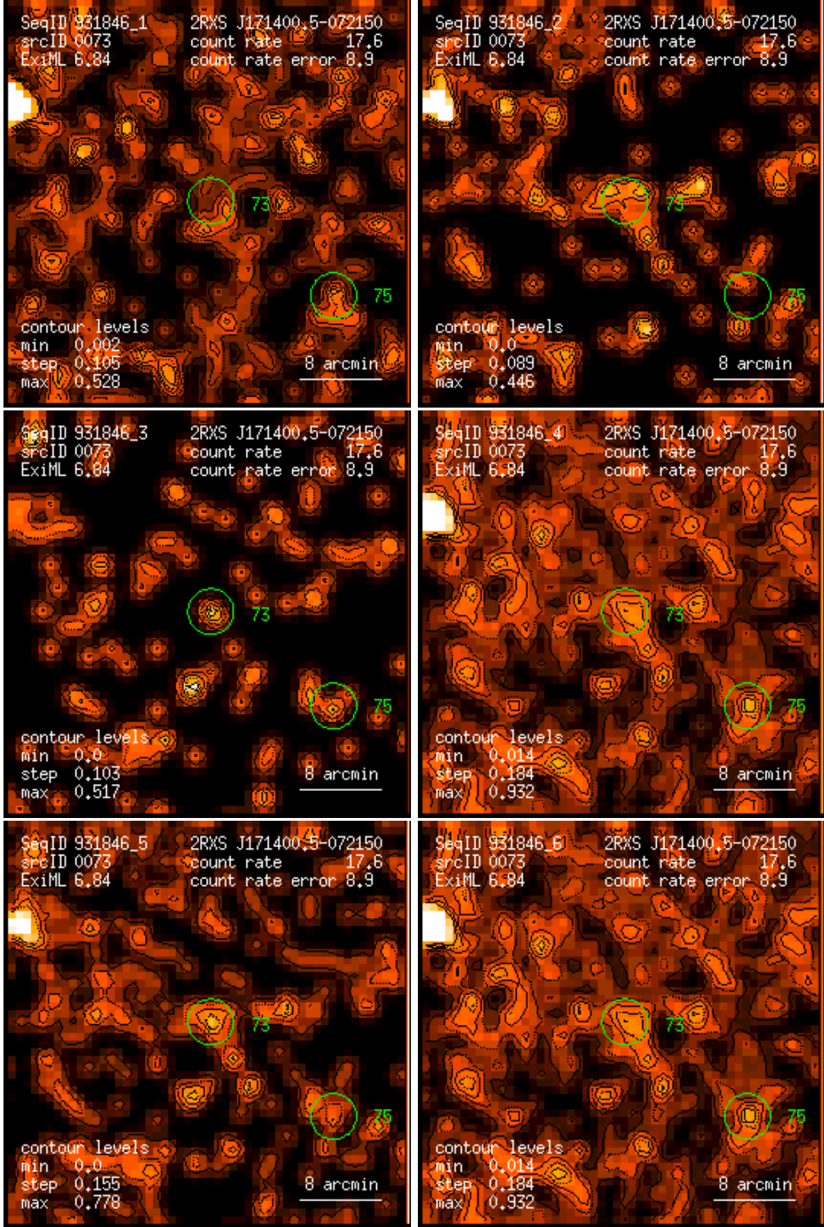
Figure 73: RASS 931846: detection 0073: band rate images, Gaussian filter: (1) PSPC channels 11 – 41, (2) 52 – 90, (3) 91 – 201, (4) 11 – 235, (5) 52 – 201, (6) 11 – 201. Broad band rates in counts/ks. Band rate contour levels in counts/ks/arcmin 2 .
