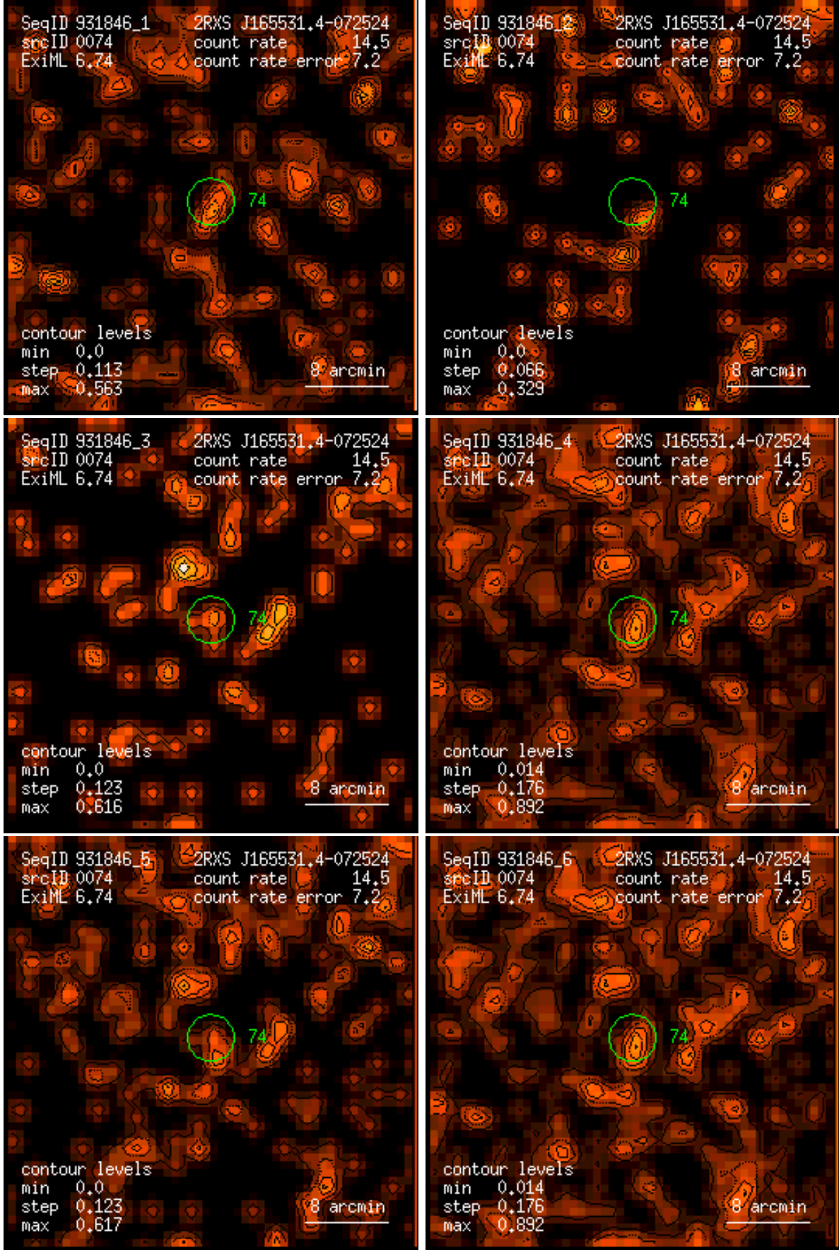
Figure 74: RASS 931846: detection 0074: band rate images, Gaussian filter: (1) PSPC channels 11 – 41, (2) 52 – 90, (3) 91 – 201, (4) 11 – 235, (5) 52 – 201, (6) 11 – 201. Broad band rates in counts/ks. Band rate contour levels in counts/ks/arcmin 2 .
