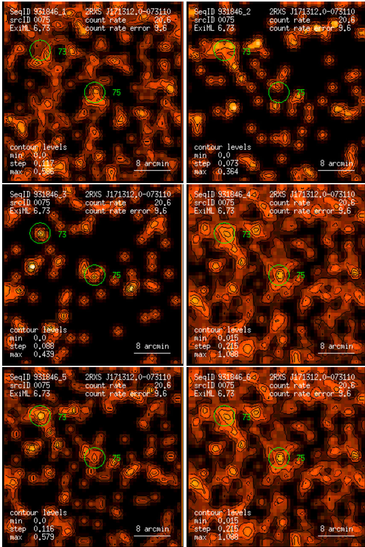
Figure 75: RASS 931846: detection 0075: band rate images, Gaussian filter: (1) PSPC channels 11 – 41, (2) 52 – 90, (3) 91 – 201, (4) 11 – 235, (5) 52 – 201, (6) 11 – 201. Broad band rates in counts/ks. Band rate contour levels in counts/ks/arcmin 2 .
