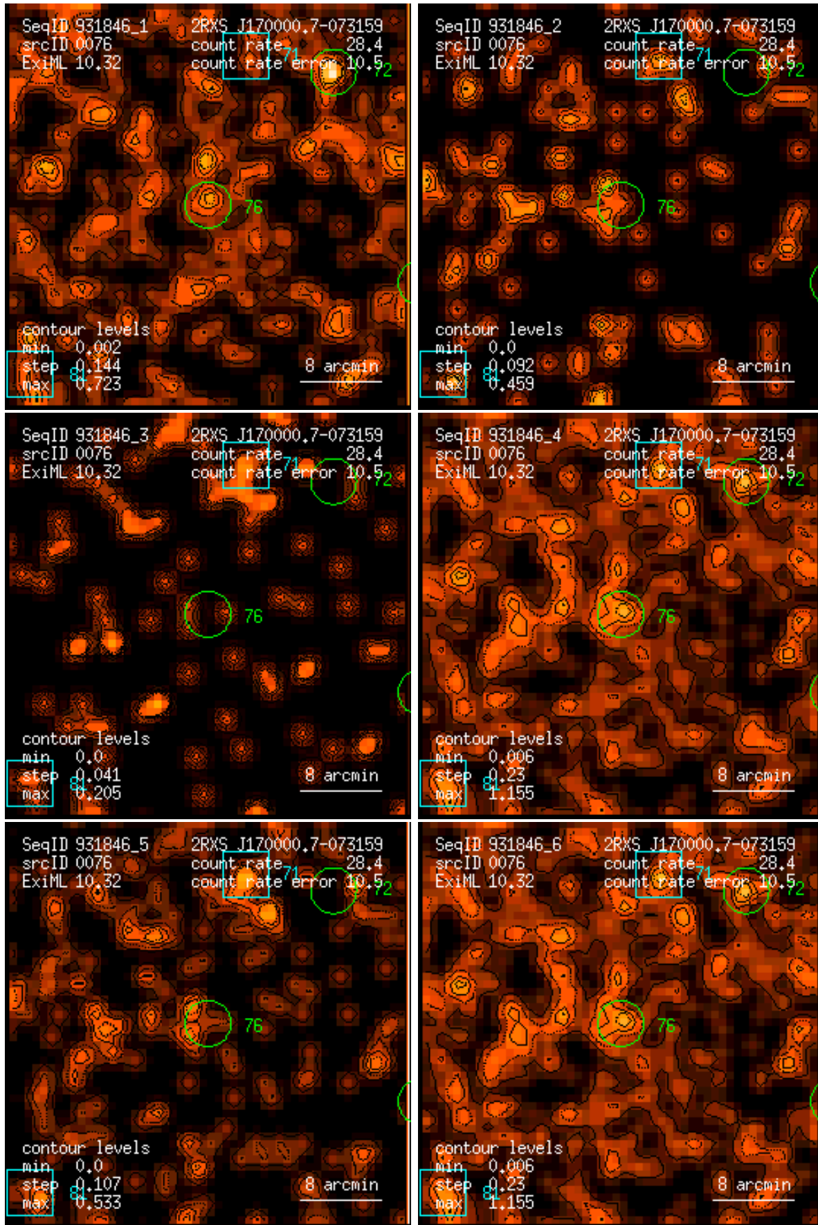
Figure 76: RASS 931846: detection 0076: band rate images, Gaussian filter: (1) PSPC channels 11 – 41, (2) 52 – 90, (3) 91 – 201, (4) 11 – 235, (5) 52 – 201, (6) 11 – 201. Broad band rates in counts/ks. Band rate contour levels in counts/ks/arcmin 2 .
