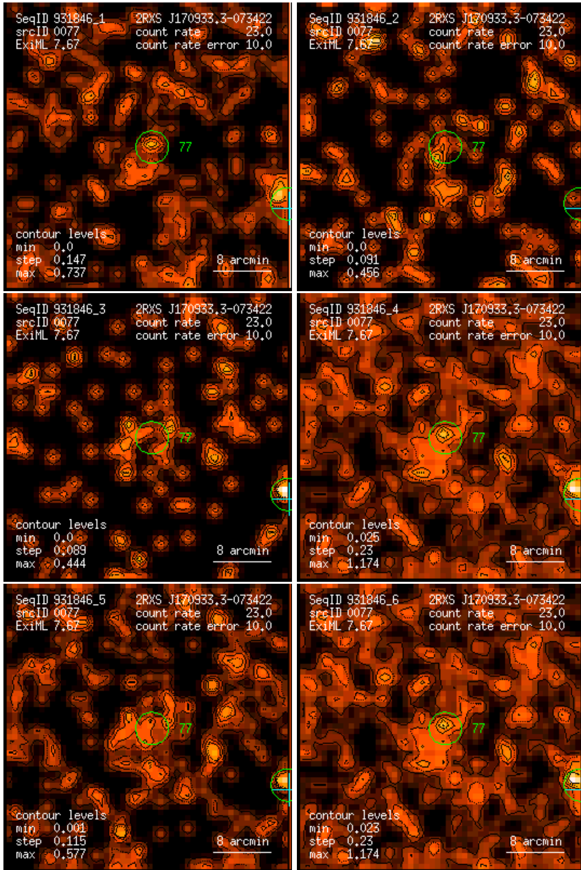
Figure 77: RASS 931846: detection 0077: band rate images, Gaussian filter: (1) PSPC channels 11 – 41, (2) 52 – 90, (3) 91 – 201, (4) 11 – 235, (5) 52 – 201, (6) 11 – 201. Broad band rates in counts/ks. Band rate contour levels in counts/ks/arcmin 2 .
