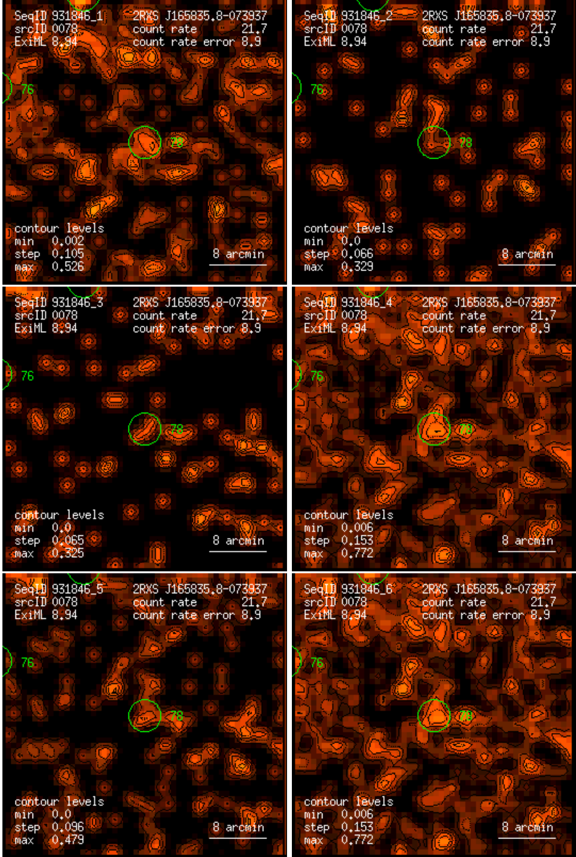
Figure 78: RASS 931846: detection 0078: band rate images, Gaussian filter: (1) PSPC channels 11 – 41, (2) 52 – 90, (3) 91 – 201, (4) 11 – 235, (5) 52 – 201, (6) 11 – 201. Broad band rates in counts/ks. Band rate contour levels in counts/ks/arcmin 2 .
