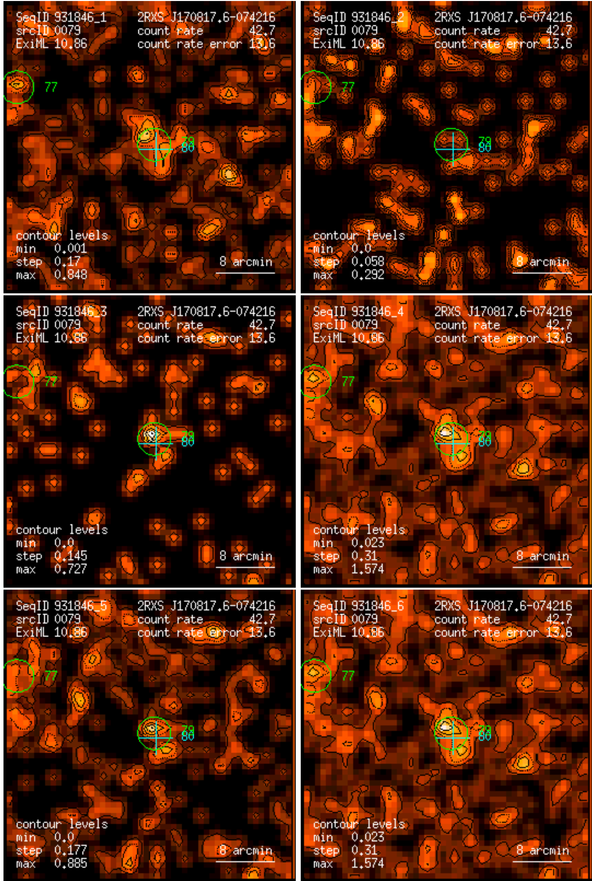
Figure 79: RASS 931846: detection 0079: band rate images, Gaussian filter: (1) PSPC channels 11 – 41, (2) 52 – 90, (3) 91 – 201, (4) 11 – 235, (5) 52 – 201, (6) 11 – 201. Broad band rates in counts/ks. Band rate contour levels in counts/ks/arcmin 2 .
