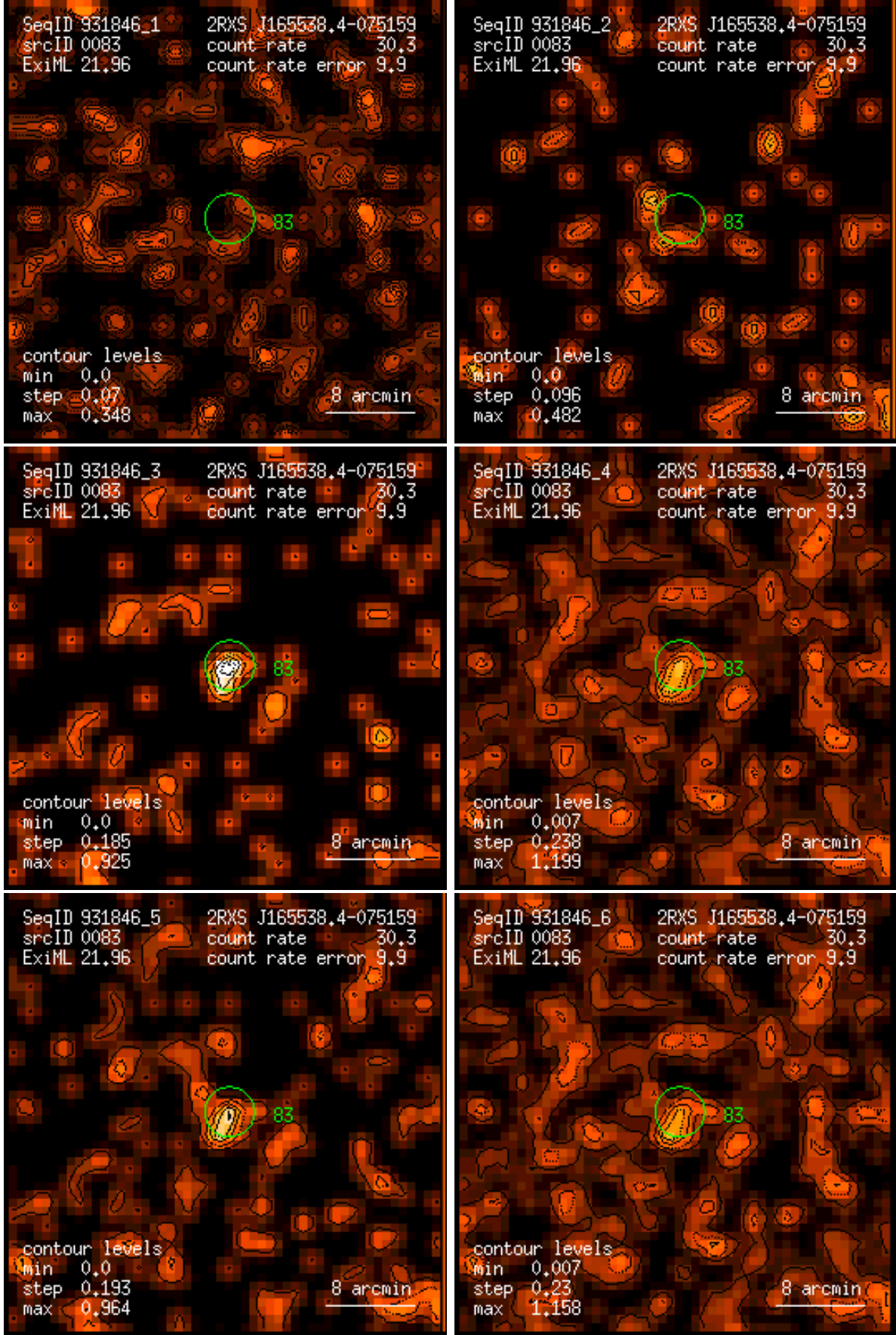
Figure 83: RASS 931846: detection 0083: band rate images, Gaussian filter: (1) PSPC channels 11 – 41, (2) 52 – 90, (3) 91 – 201, (4) 11 – 235, (5) 52 – 201, (6) 11 – 201. Broad band rates in counts/ks. Band rate contour levels in counts/ks/arcmin 2 .
