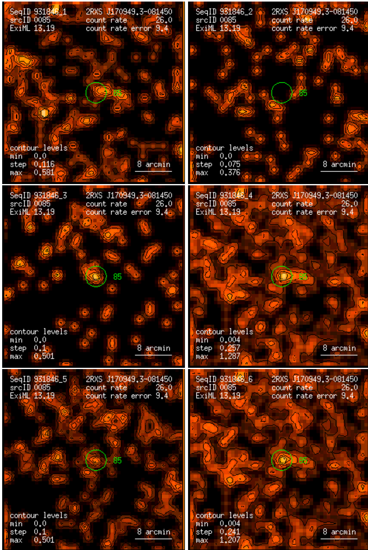
Figure 85: RASS 931846: detection 0085: band rate images, Gaussian filter: (1) PSPC channels 11 – 41, (2) 52 – 90, (3) 91 – 201, (4) 11 – 235, (5) 52 – 201, (6) 11 – 201. Broad band rates in counts/ks. Band rate contour levels in counts/ks/arcmin 2 .
