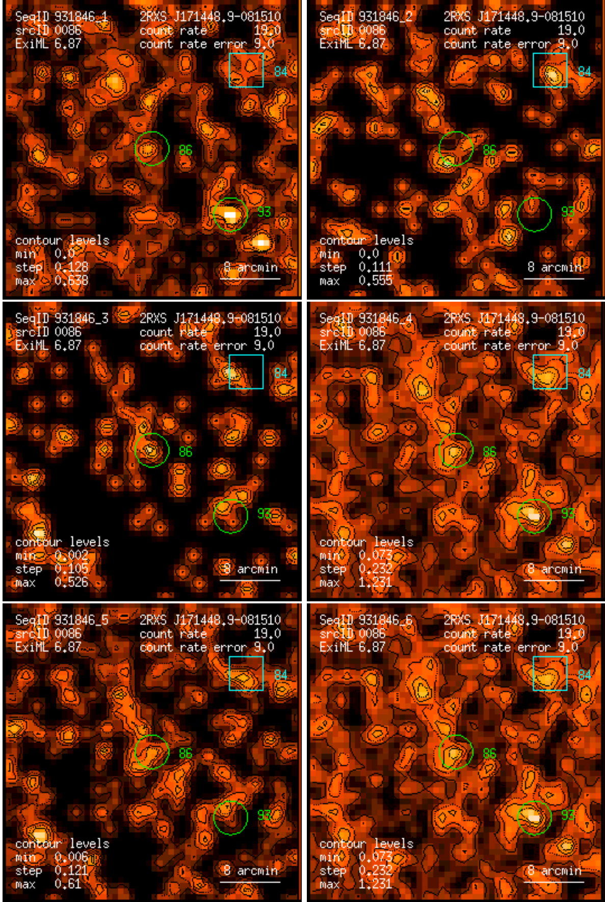
Figure 86: RASS 931846: detection 0086: band rate images, Gaussian filter: (1) PSPC channels 11 – 41, (2) 52 – 90, (3) 91 – 201, (4) 11 – 235, (5) 52 – 201, (6) 11 – 201. Broad band rates in counts/ks. Band rate contour levels in counts/ks/arcmin 2 .
