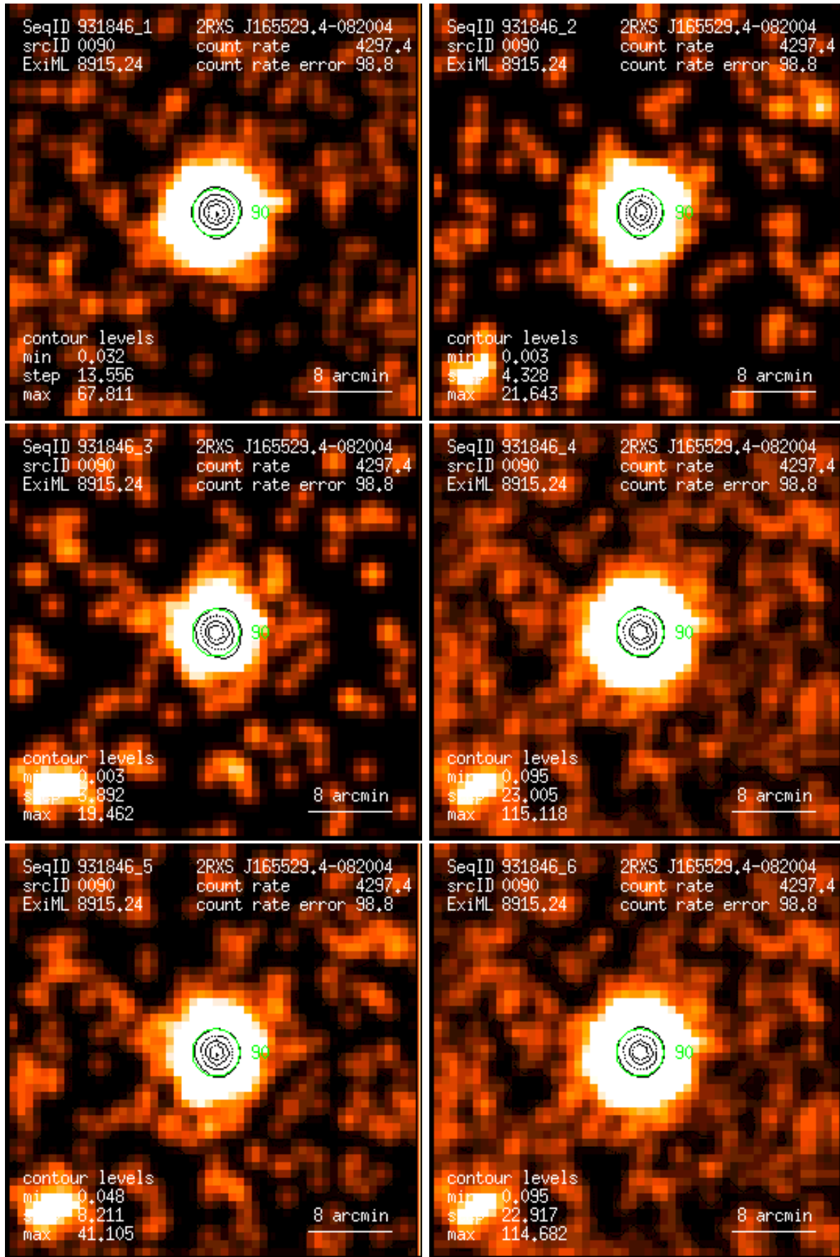
Figure 90: RASS 931846: detection 0090: band rate images, Gaussian filter: (1) PSPC channels 11 – 41, (2) 52 – 90, (3) 91 – 201, (4) 11 – 235, (5) 52 – 201, (6) 11 – 201. Broad band rates in counts/ks. Band rate contour levels in counts/ks/arcmin 2 .
