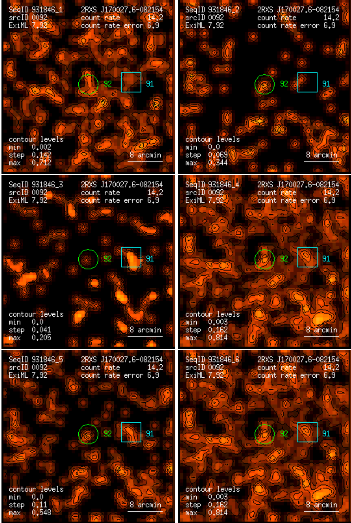
Figure 92: RASS 931846: detection 0092: band rate images, Gaussian filter: (1) PSPC channels 11 – 41, (2) 52 – 90, (3) 91 – 201, (4) 11 – 235, (5) 52 – 201, (6) 11 – 201. Broad band rates in counts/ks. Band rate contour levels in counts/ks/arcmin 2 .
