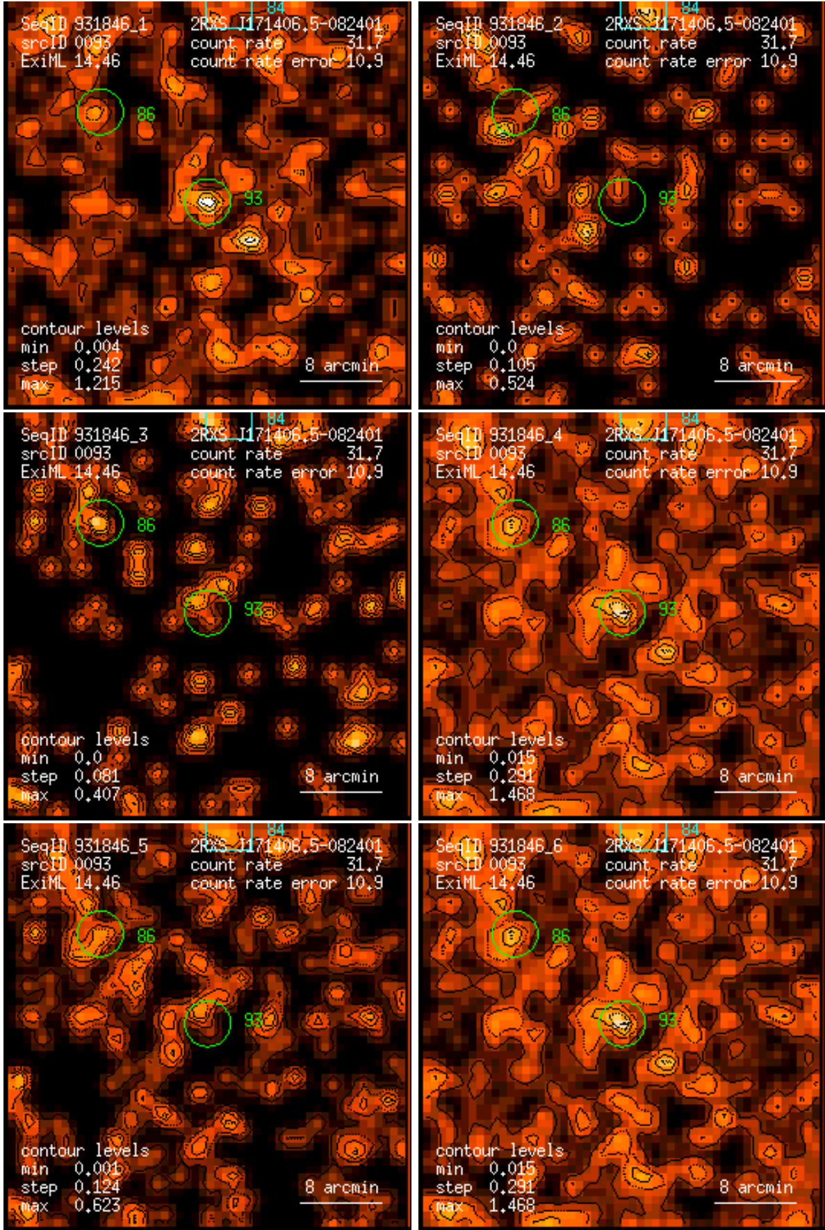
Figure 93: RASS 931846: detection 0093: band rate images, Gaussian filter: (1) PSPC channels 11 – 41, (2) 52 – 90, (3) 91 – 201, (4) 11 – 235, (5) 52 – 201, (6) 11 – 201. Broad band rates in counts/ks. Band rate contour levels in counts/ks/arcmin 2 .
