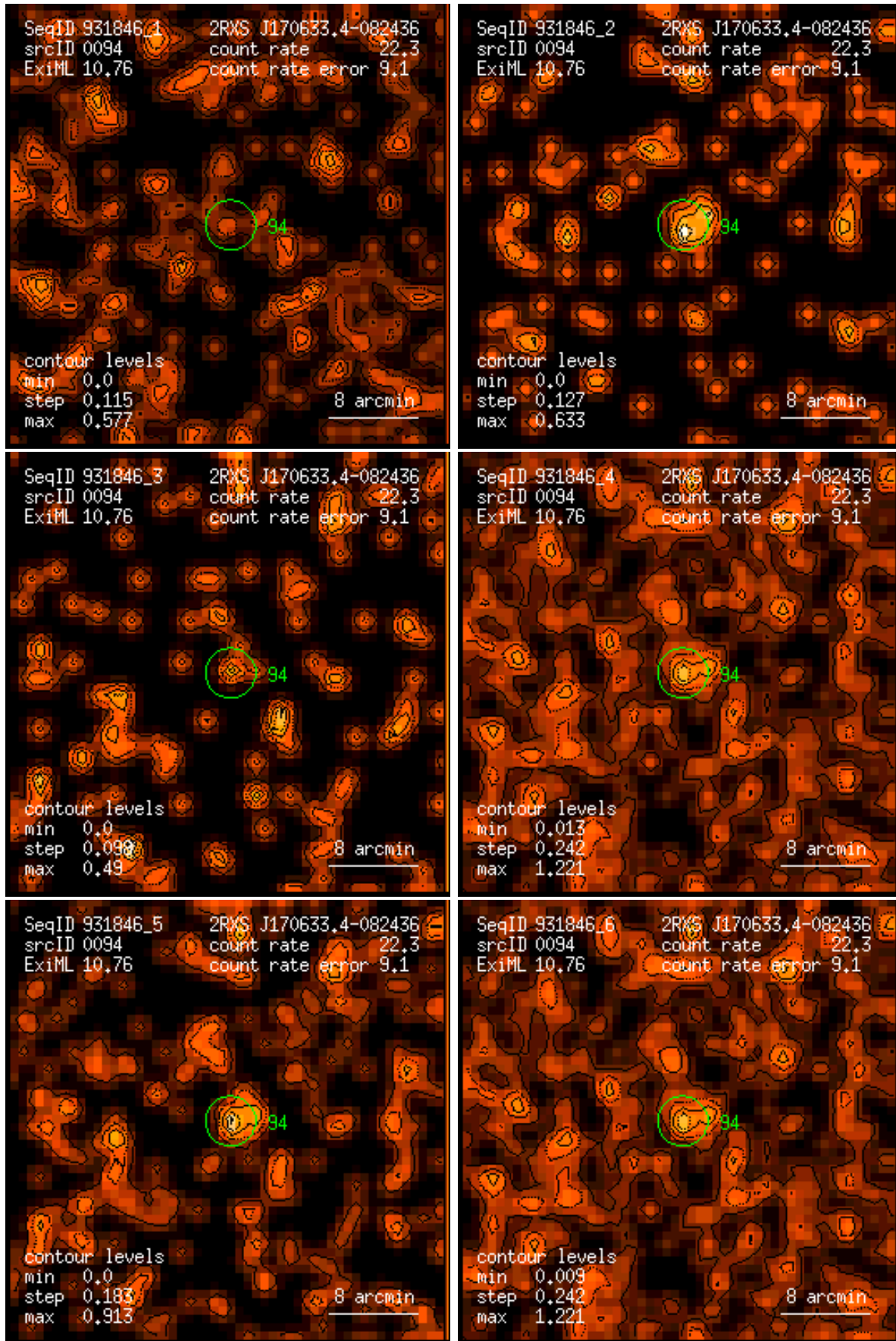
Figure 94: RASS 931846: detection 0094: band rate images, Gaussian filter: (1) PSPC channels 11 – 41, (2) 52 – 90, (3) 91 – 201, (4) 11 – 235, (5) 52 – 201, (6) 11 – 201. Broad band rates in counts/ks. Band rate contour levels in counts/ks/arcmin 2 .
