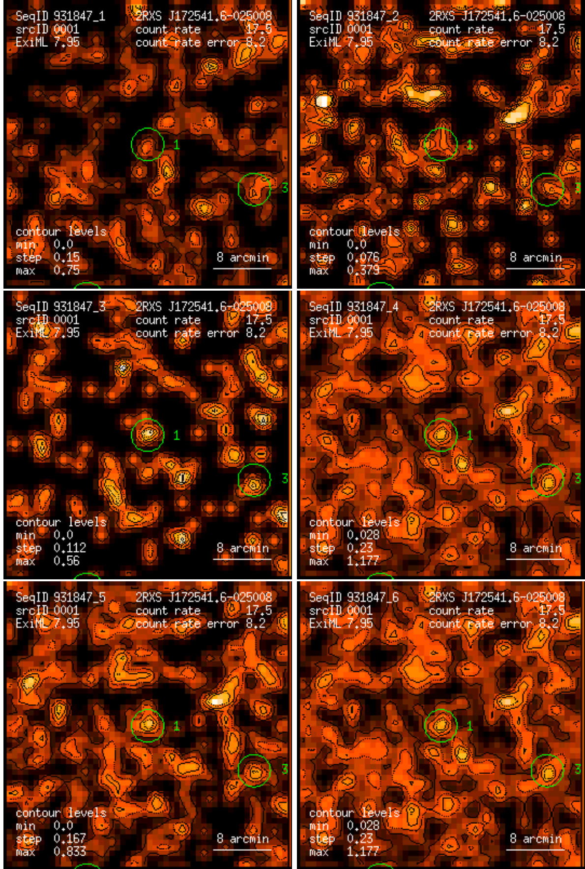
Figure 1: RASS 931847: detection 0001: band rate images, Gaussian filter: (1) PSPC channels 11 – 41, (2) 52 – 90, (3) 91 – 201, (4) 11 – 235, (5) 52 – 201, (6) 11 – 201. Broad band rates in counts/ks. Band rate contour levels in counts/ks/arcmin 2 .
