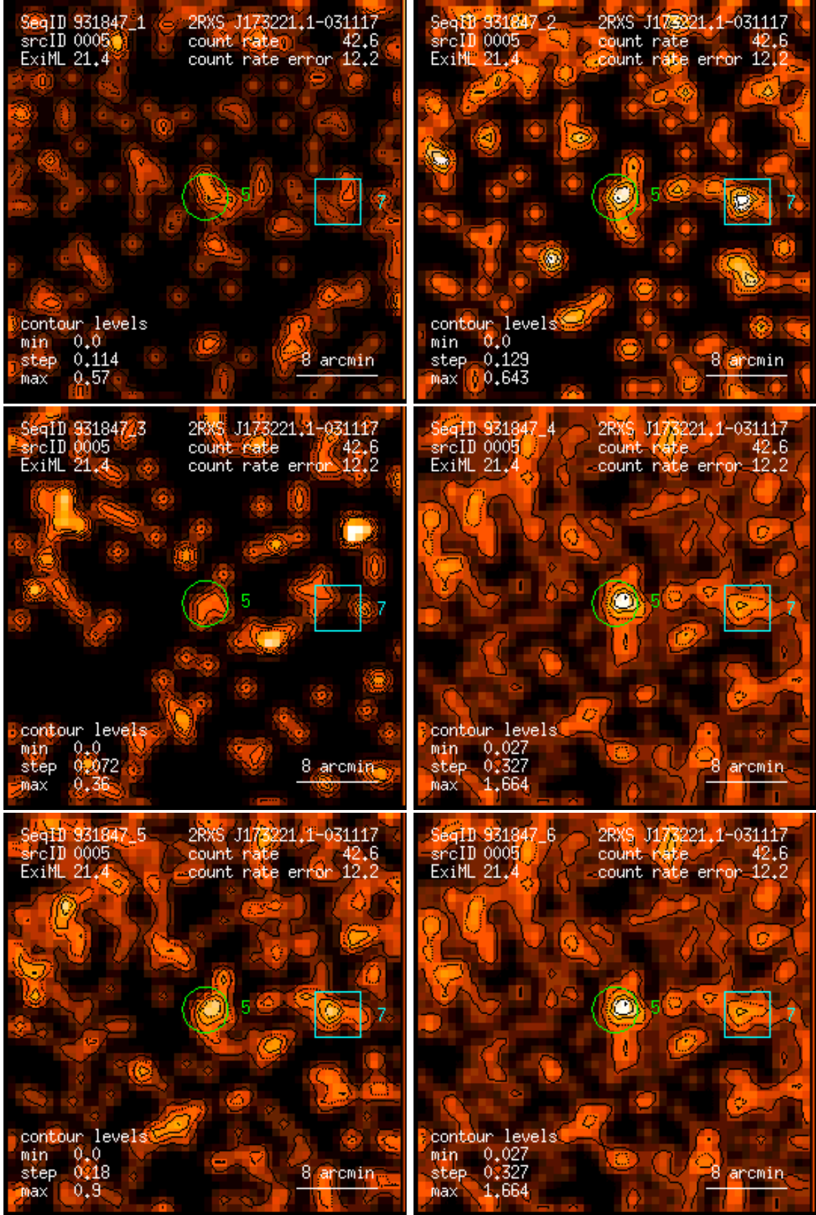
Figure 5: RASS 931847: detection 0005: band rate images, Gaussian filter: (1) PSPC channels 11 – 41, (2) 52 – 90, (3) 91 – 201, (4) 11 – 235, (5) 52 – 201, (6) 11 – 201. Broad band rates in counts/ks. Band rate contour levels in counts/ks/arcmin 2 .
