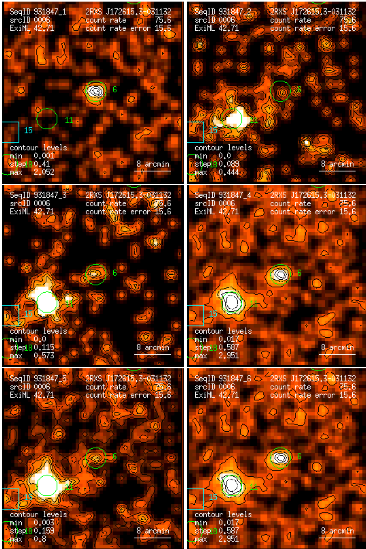
Figure 6: RASS 931847: detection 0006: band rate images, Gaussian filter: (1) PSPC channels 11 – 41, (2) 52 – 90, (3) 91 – 201, (4) 11 – 235, (5) 52 – 201, (6) 11 – 201. Broad band rates in counts/ks. Band rate contour levels in counts/ks/arcmin 2 .
