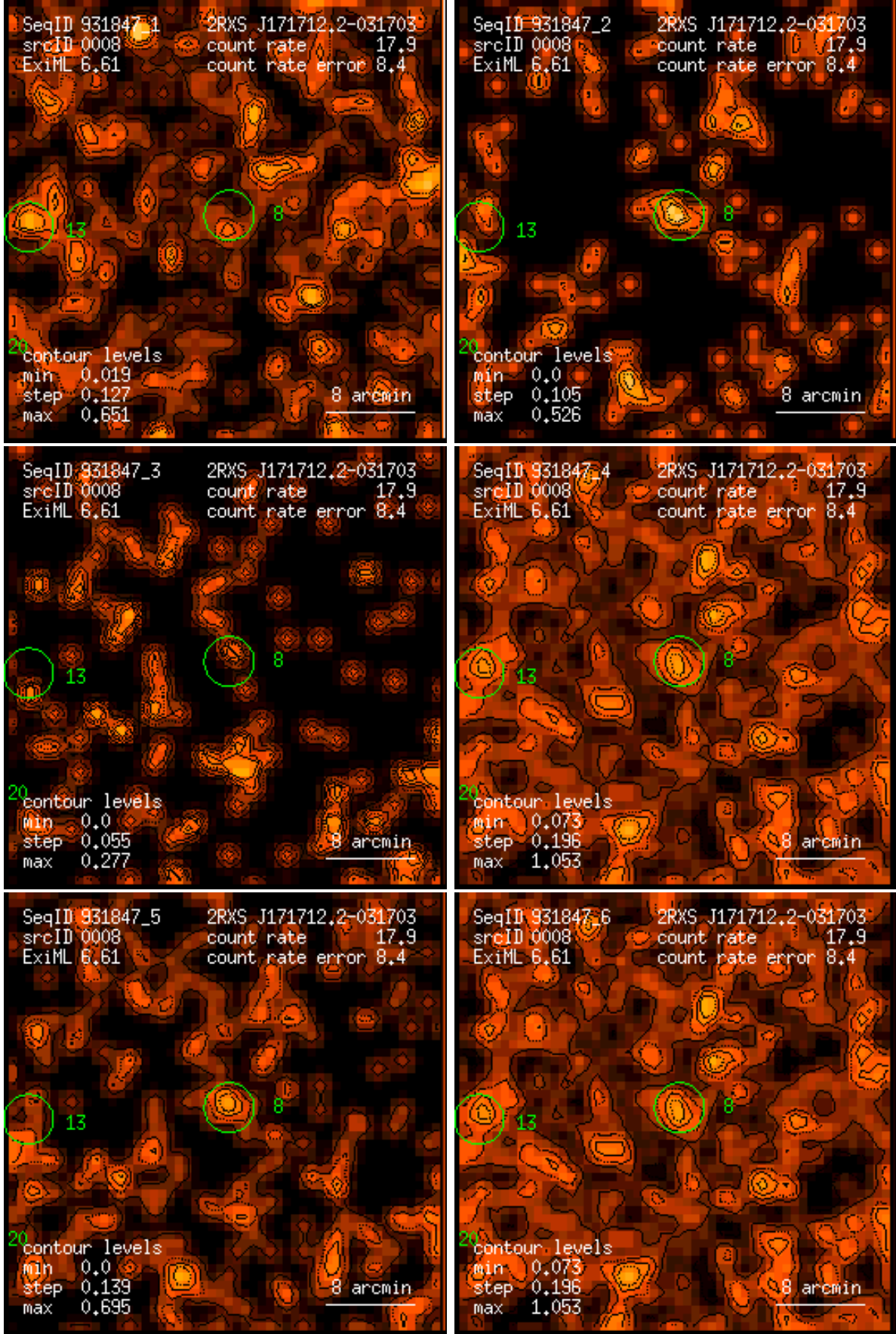
Figure 8: RASS 931847: detection 0008: band rate images, Gaussian filter: (1) PSPC channels 11 – 41, (2) 52 – 90, (3) 91 – 201, (4) 11 – 235, (5) 52 – 201, (6) 11 – 201. Broad band rates in counts/ks. Band rate contour levels in counts/ks/arcmin 2 .
