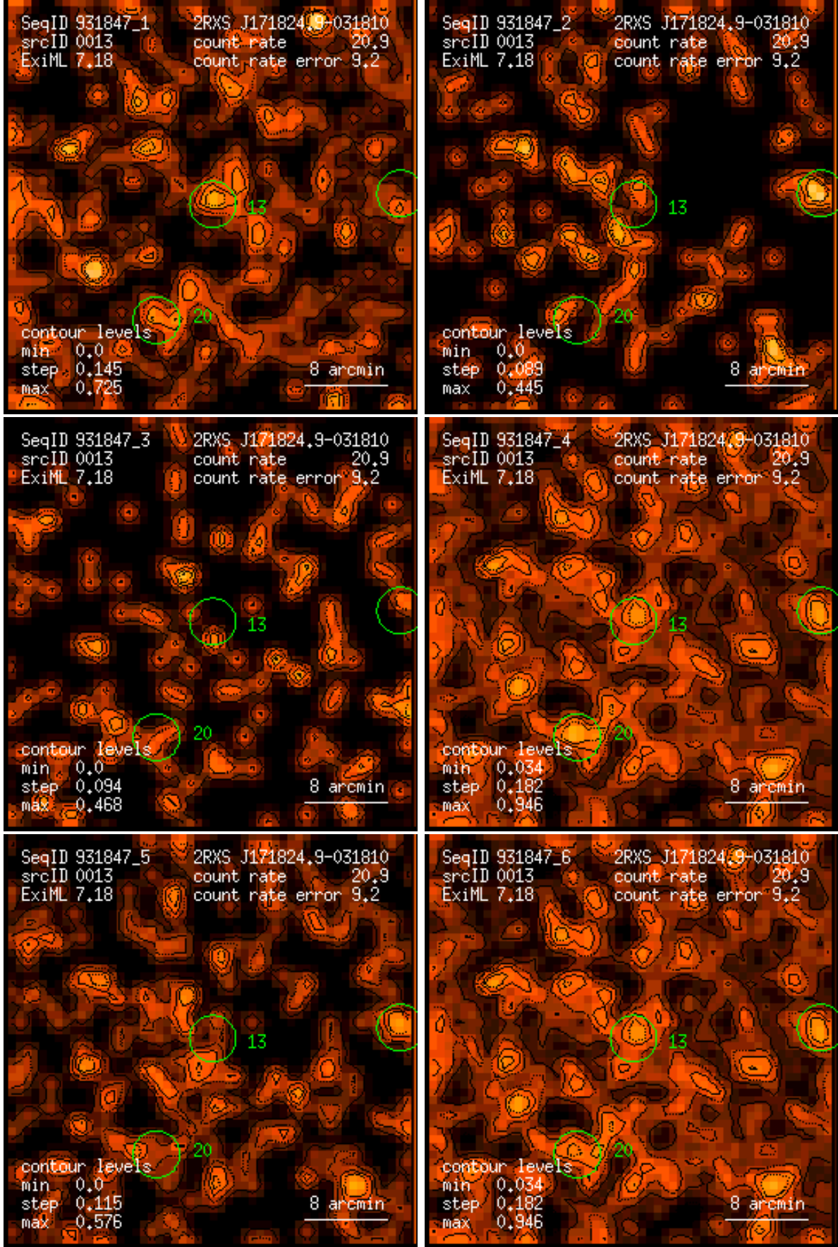
Figure 13: RASS 931847: detection 0013: band rate images, Gaussian filter: (1) PSPC channels 11 – 41, (2) 52 – 90, (3) 91 – 201, (4) 11 – 235, (5) 52 – 201, (6) 11 – 201. Broad band rates in counts/ks. Band rate contour levels in counts/ks/arcmin 2 .
