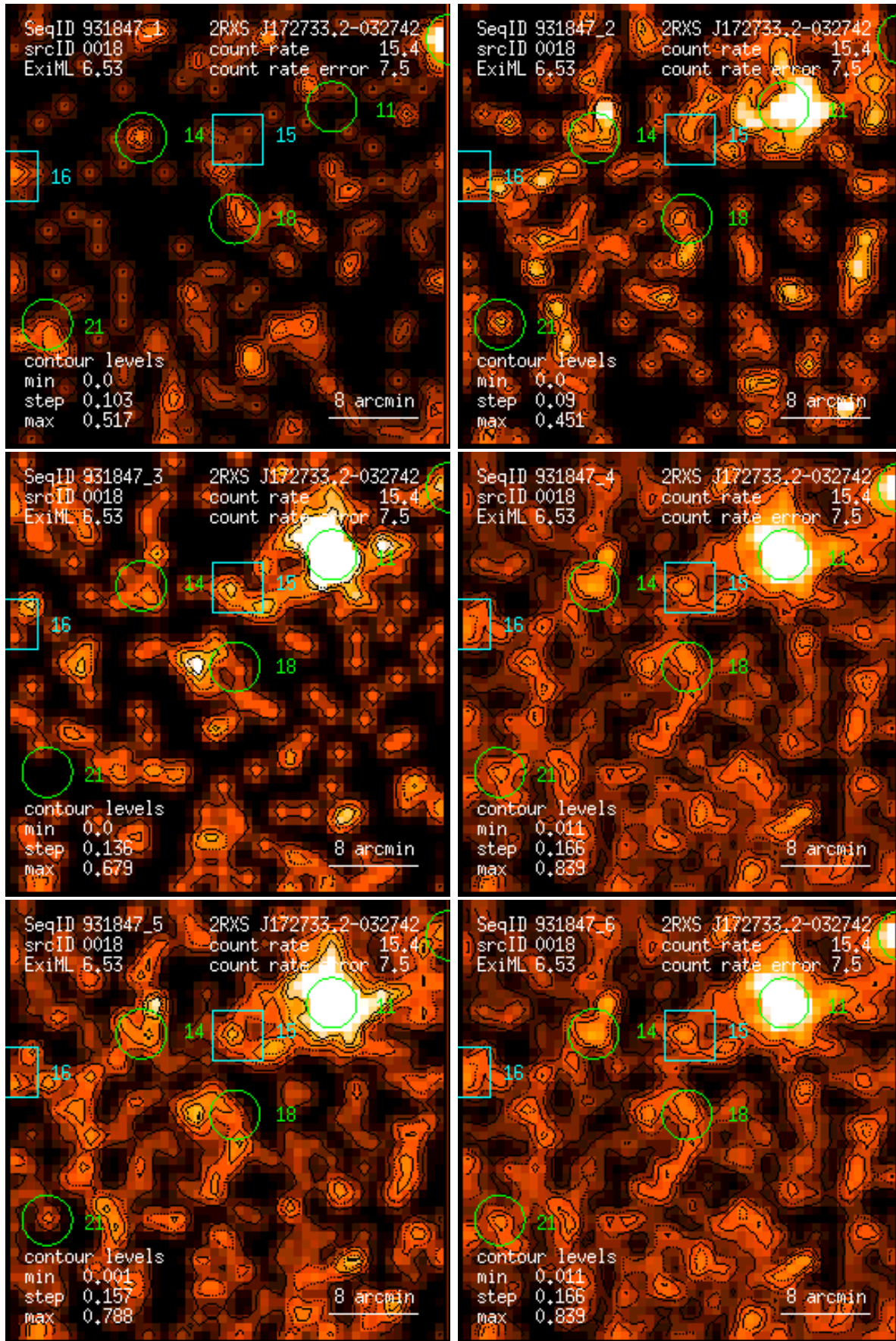
Figure 18: RASS 931847: detection 0018: band rate images, Gaussian filter: (1) PSPC channels 11 – 41, (2) 52 – 90, (3) 91 – 201, (4) 11 – 235, (5) 52 – 201, (6) 11 – 201. Broad band rates in counts/ks. Band rate contour levels in counts/ks/arcmin 2 .
