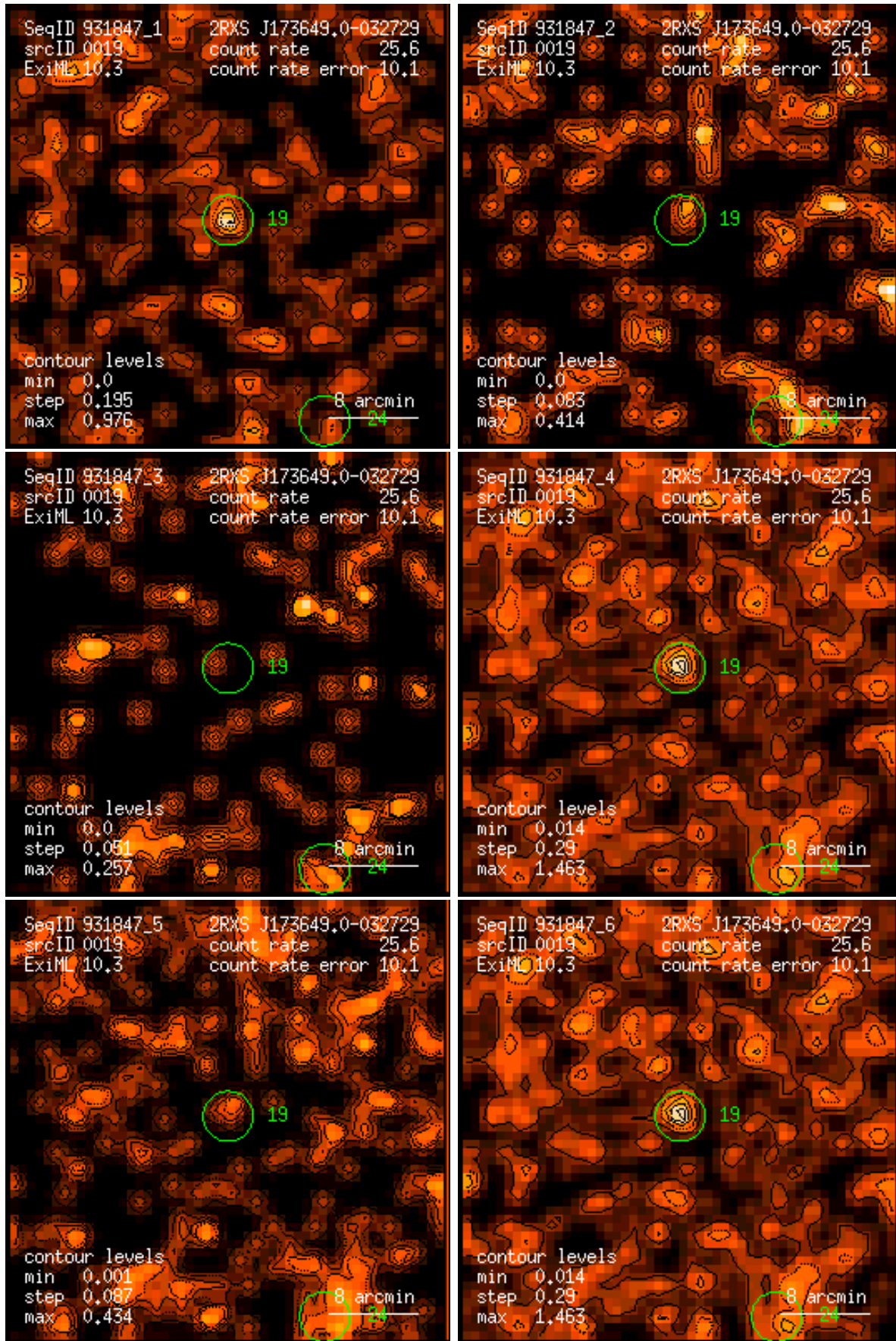
Figure 19: RASS 931847: detection 0019: band rate images, Gaussian filter: (1) PSPC channels 11 – 41, (2) 52 – 90, (3) 91 – 201, (4) 11 – 235, (5) 52 – 201, (6) 11 – 201. Broad band rates in counts/ks. Band rate contour levels in counts/ks/arcmin 2 .
