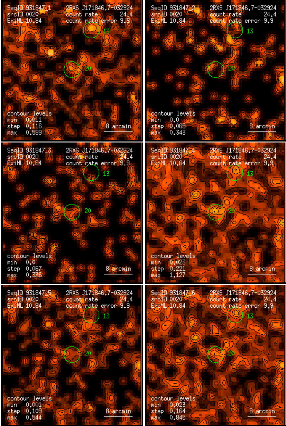
Figure 20: RASS 931847: detection 0020: band rate images, Gaussian filter: (1) PSPC channels 11 – 41, (2) 52 – 90, (3) 91 – 201, (4) 11 – 235, (5) 52 – 201, (6) 11 – 201. Broad band rates in counts/ks. Band rate contour levels in counts/ks/arcmin 2 .
