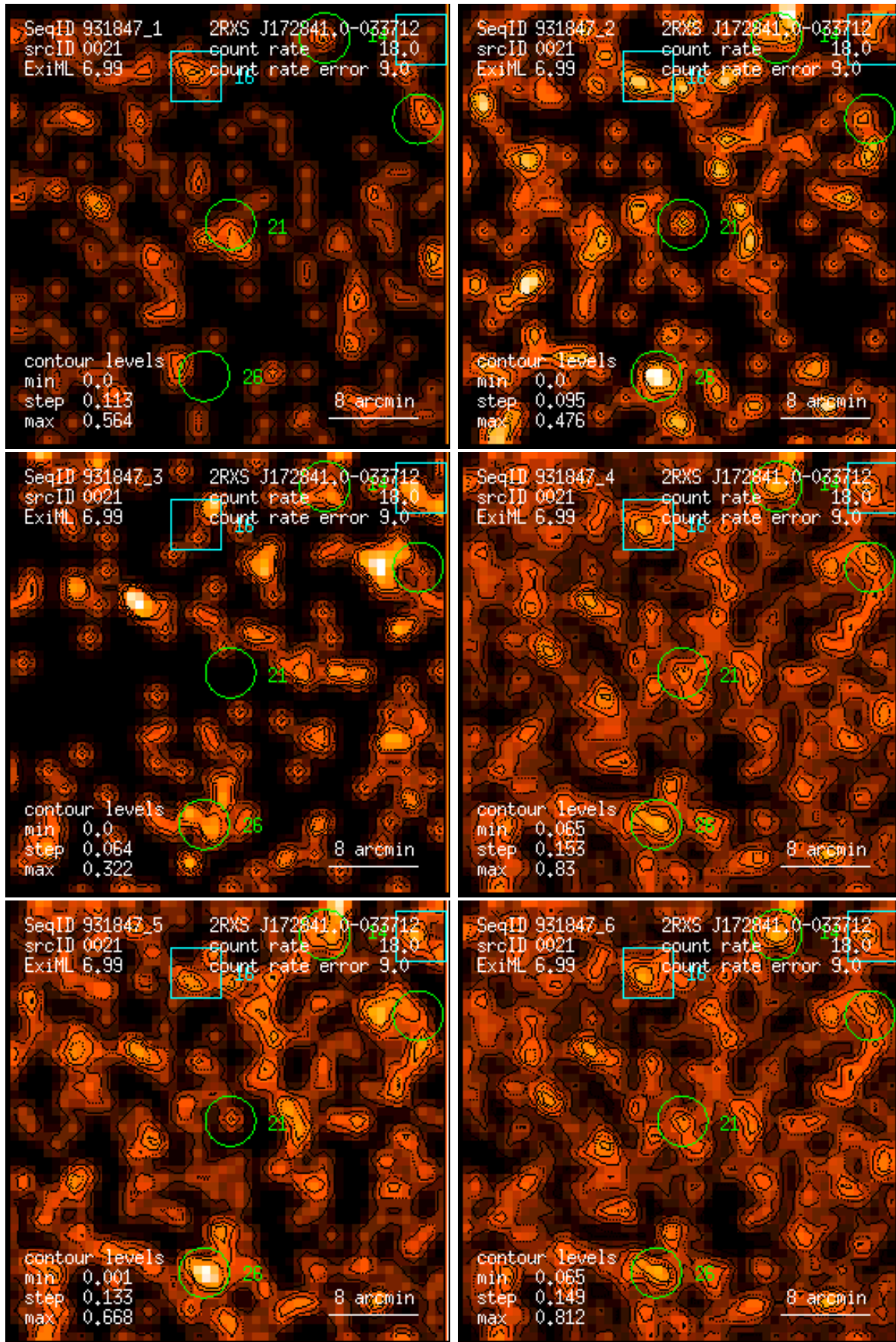
Figure 21: RASS 931847: detection 0021: band rate images, Gaussian filter: (1) PSPC channels 11 – 41, (2) 52 – 90, (3) 91 – 201, (4) 11 – 235, (5) 52 – 201, (6) 11 – 201. Broad band rates in counts/ks. Band rate contour levels in counts/ks/arcmin 2 .
