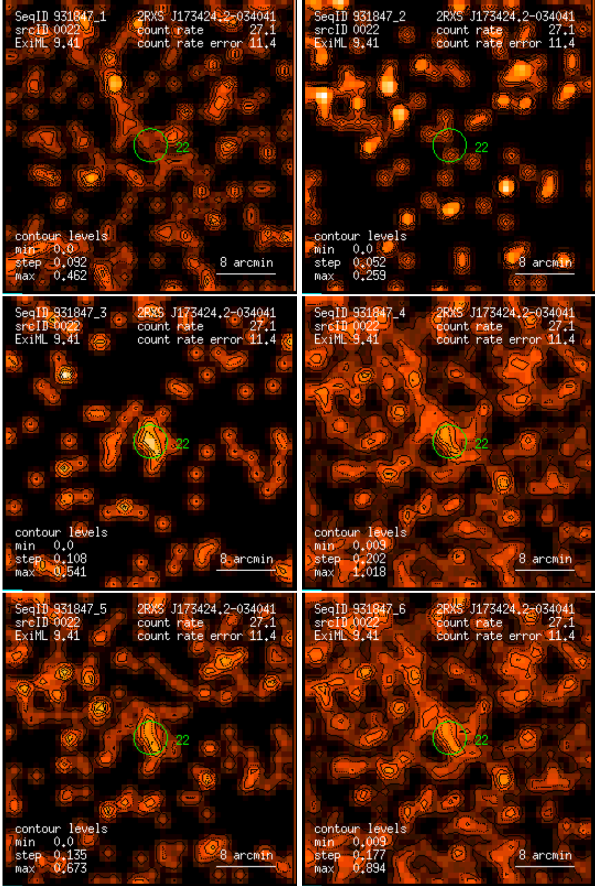
Figure 22: RASS 931847: detection 0022: band rate images, Gaussian filter: (1) PSPC channels 11 – 41, (2) 52 – 90, (3) 91 – 201, (4) 11 – 235, (5) 52 – 201, (6) 11 – 201. Broad band rates in counts/ks. Band rate contour levels in counts/ks/arcmin 2 .
