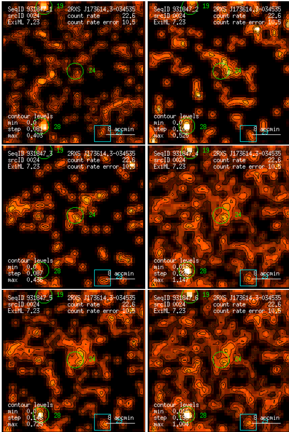
Figure 24: RASS 931847: detection 0024: band rate images, Gaussian filter: (1) PSPC channels 11 – 41, (2) 52 – 90, (3) 91 – 201, (4) 11 – 235, (5) 52 – 201, (6) 11 – 201. Broad band rates in counts/ks. Band rate contour levels in counts/ks/arcmin 2 .
