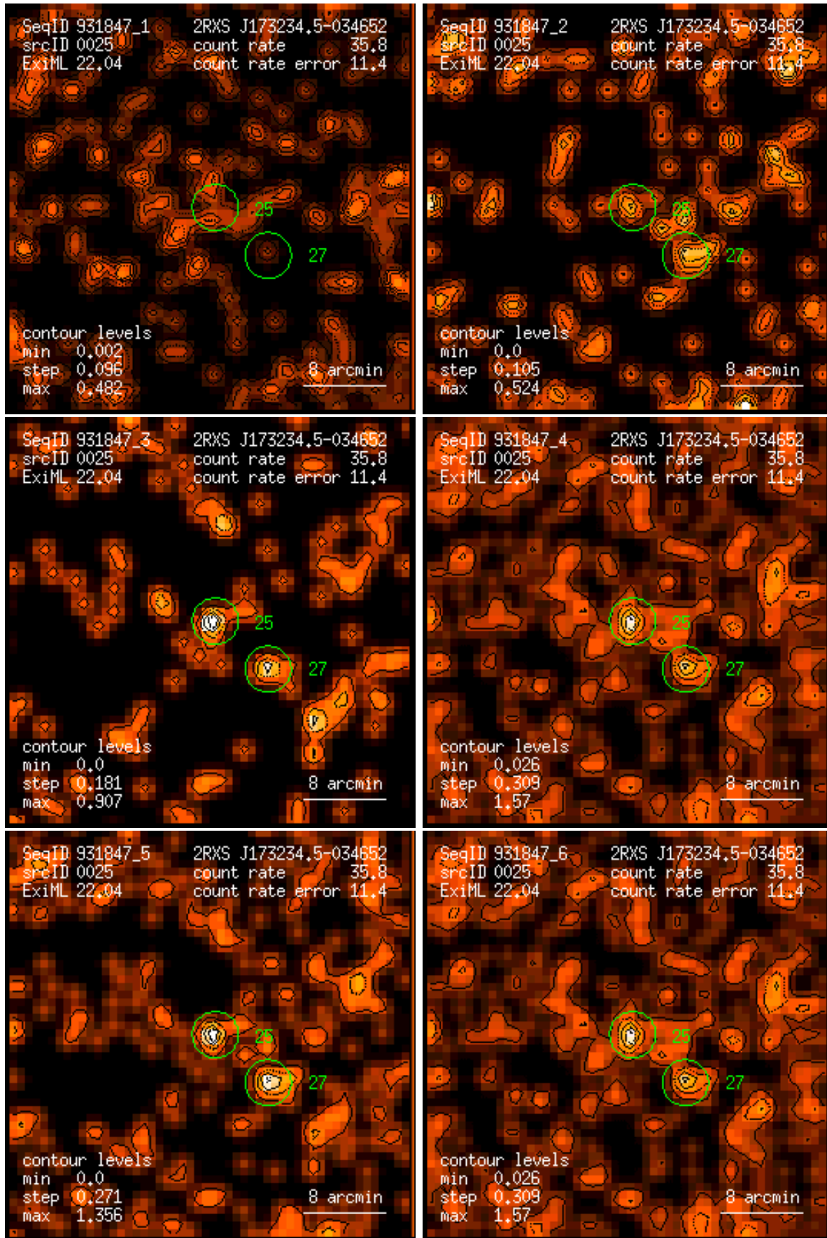
Figure 25: RASS 931847: detection 0025: band rate images, Gaussian filter: (1) PSPC channels 11 – 41, (2) 52 – 90, (3) 91 – 201, (4) 11 – 235, (5) 52 – 201, (6) 11 – 201. Broad band rates in counts/ks. Band rate contour levels in counts/ks/arcmin 2 .
