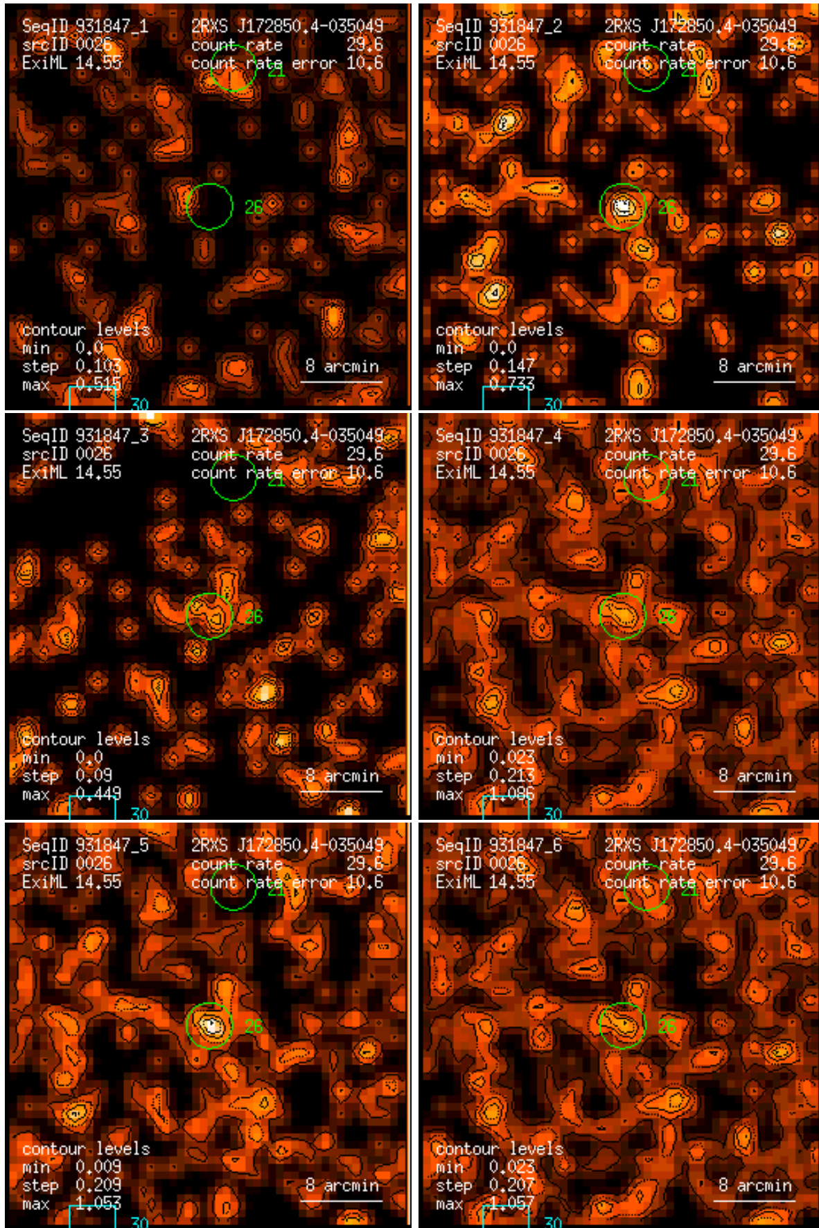
Figure 26: RASS 931847: detection 0026: band rate images, Gaussian filter: (1) PSPC channels 11 – 41, (2) 52 – 90, (3) 91 – 201, (4) 11 – 235, (5) 52 – 201, (6) 11 – 201. Broad band rates in counts/ks. Band rate contour levels in counts/ks/arcmin 2 .
