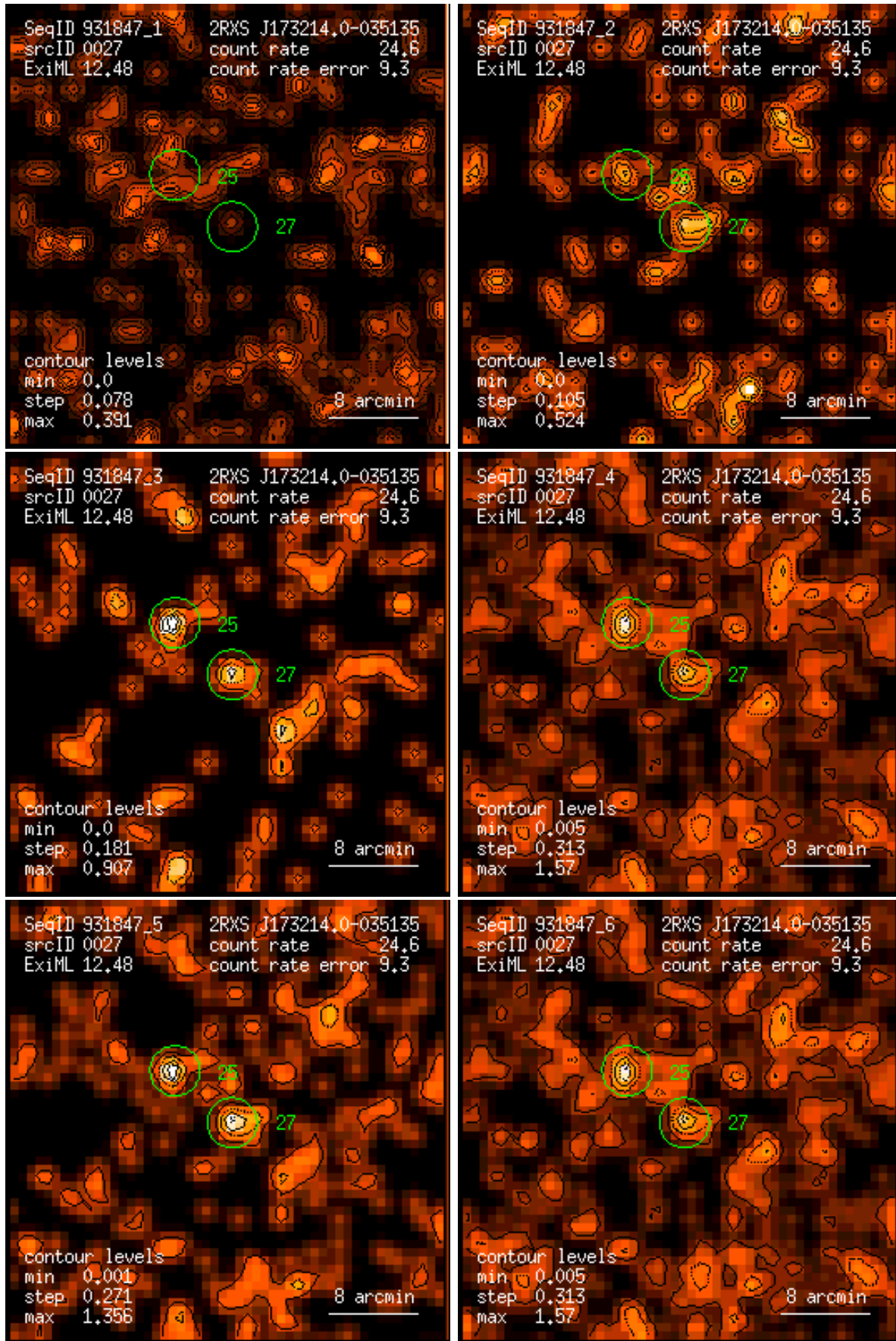
Figure 27: RASS 931847: detection 0027: band rate images, Gaussian filter: (1) PSPC channels 11 – 41, (2) 52 – 90, (3) 91 – 201, (4) 11 – 235, (5) 52 – 201, (6) 11 – 201. Broad band rates in counts/ks. Band rate contour levels in counts/ks/arcmin 2 .
