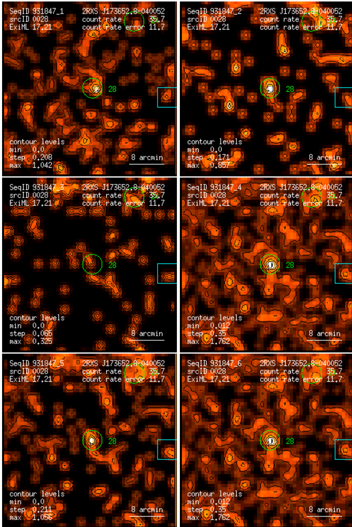
Figure 28: RASS 931847: detection 0028: band rate images, Gaussian filter: (1) PSPC channels 11 – 41, (2) 52 – 90, (3) 91 – 201, (4) 11 – 235, (5) 52 – 201, (6) 11 – 201. Broad band rates in counts/ks. Band rate contour levels in counts/ks/arcmin 2 .
