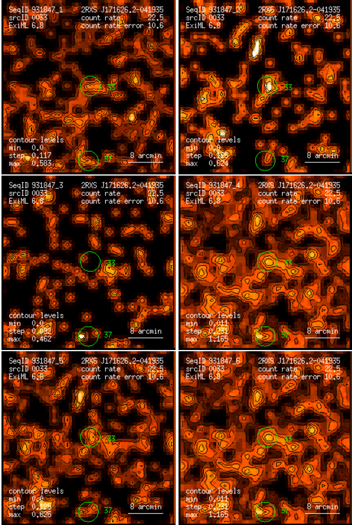
Figure 33: RASS 931847: detection 0033: band rate images, Gaussian filter: (1) PSPC channels 11 – 41, (2) 52 – 90, (3) 91 – 201, (4) 11 – 235, (5) 52 – 201, (6) 11 – 201. Broad band rates in counts/ks. Band rate contour levels in counts/ks/arcmin 2 .
