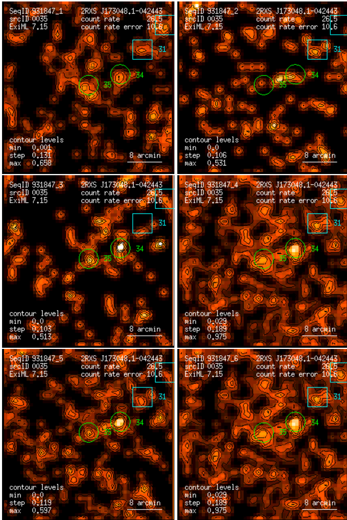
Figure 35: RASS 931847: detection 0035: band rate images, Gaussian filter: (1) PSPC channels 11 – 41, (2) 52 – 90, (3) 91 – 201, (4) 11 – 235, (5) 52 – 201, (6) 11 – 201. Broad band rates in counts/ks. Band rate contour levels in counts/ks/arcmin 2 .
