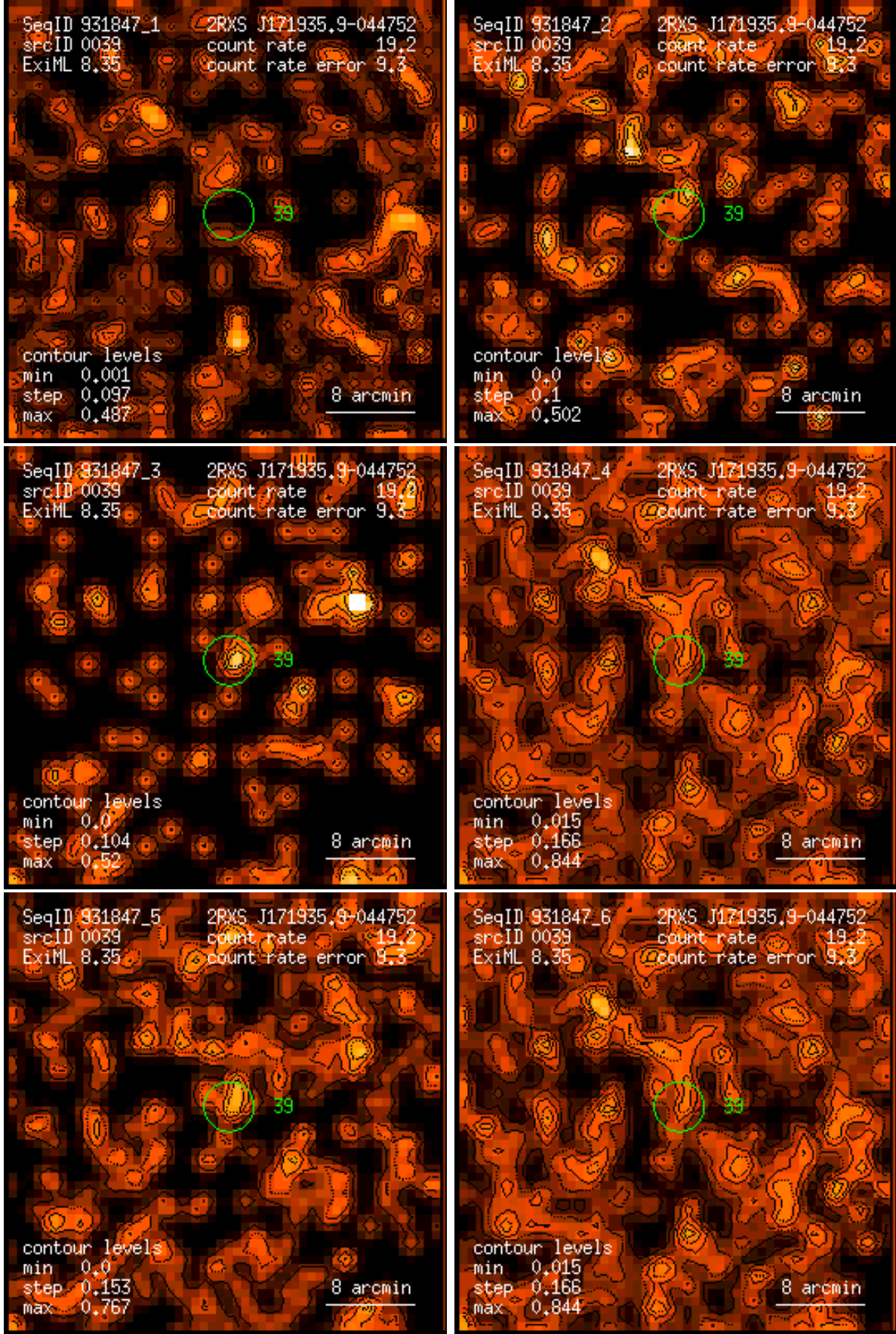
Figure 39: RASS 931847: detection 0039: band rate images, Gaussian filter: (1) PSPC channels 11 – 41, (2) 52 – 90, (3) 91 – 201, (4) 11 – 235, (5) 52 – 201, (6) 11 – 201. Broad band rates in counts/ks. Band rate contour levels in counts/ks/arcmin 2 .
