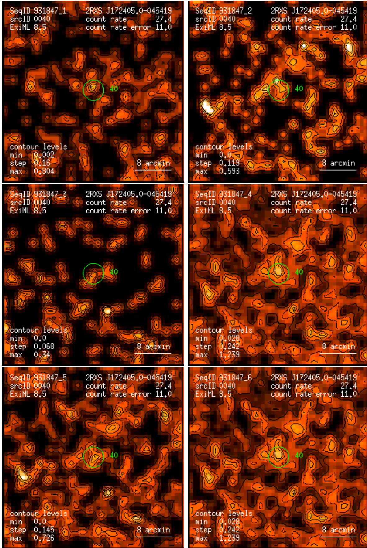
Figure 40: RASS 931847: detection 0040: band rate images, Gaussian filter: (1) PSPC channels 11 – 41, (2) 52 – 90, (3) 91 – 201, (4) 11 – 235, (5) 52 – 201, (6) 11 – 201. Broad band rates in counts/ks. Band rate contour levels in counts/ks/arcmin 2 .
