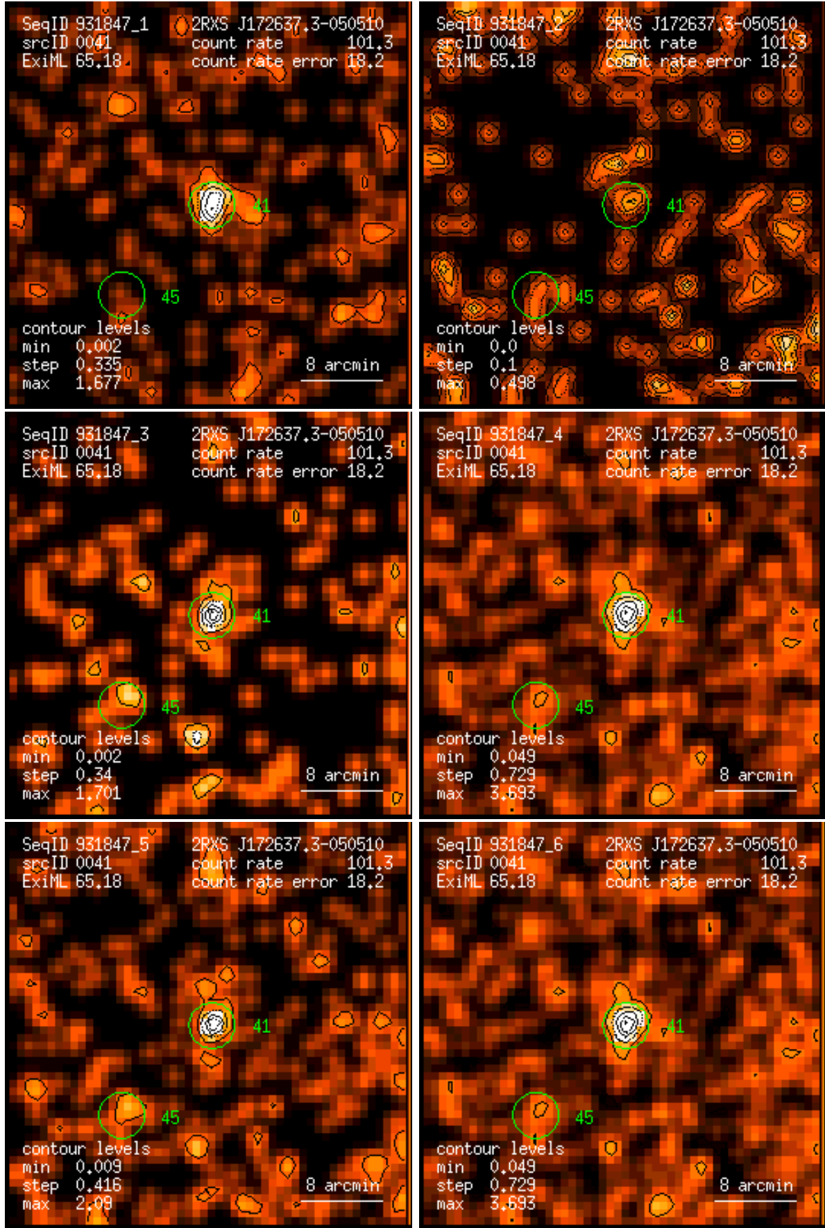
Figure 41: RASS 931847: detection 0041: band rate images, Gaussian filter: (1) PSPC channels 11 – 41, (2) 52 – 90, (3) 91 – 201, (4) 11 – 235, (5) 52 – 201, (6) 11 – 201. Broad band rates in counts/ks. Band rate contour levels in counts/ks/arcmin 2 .
