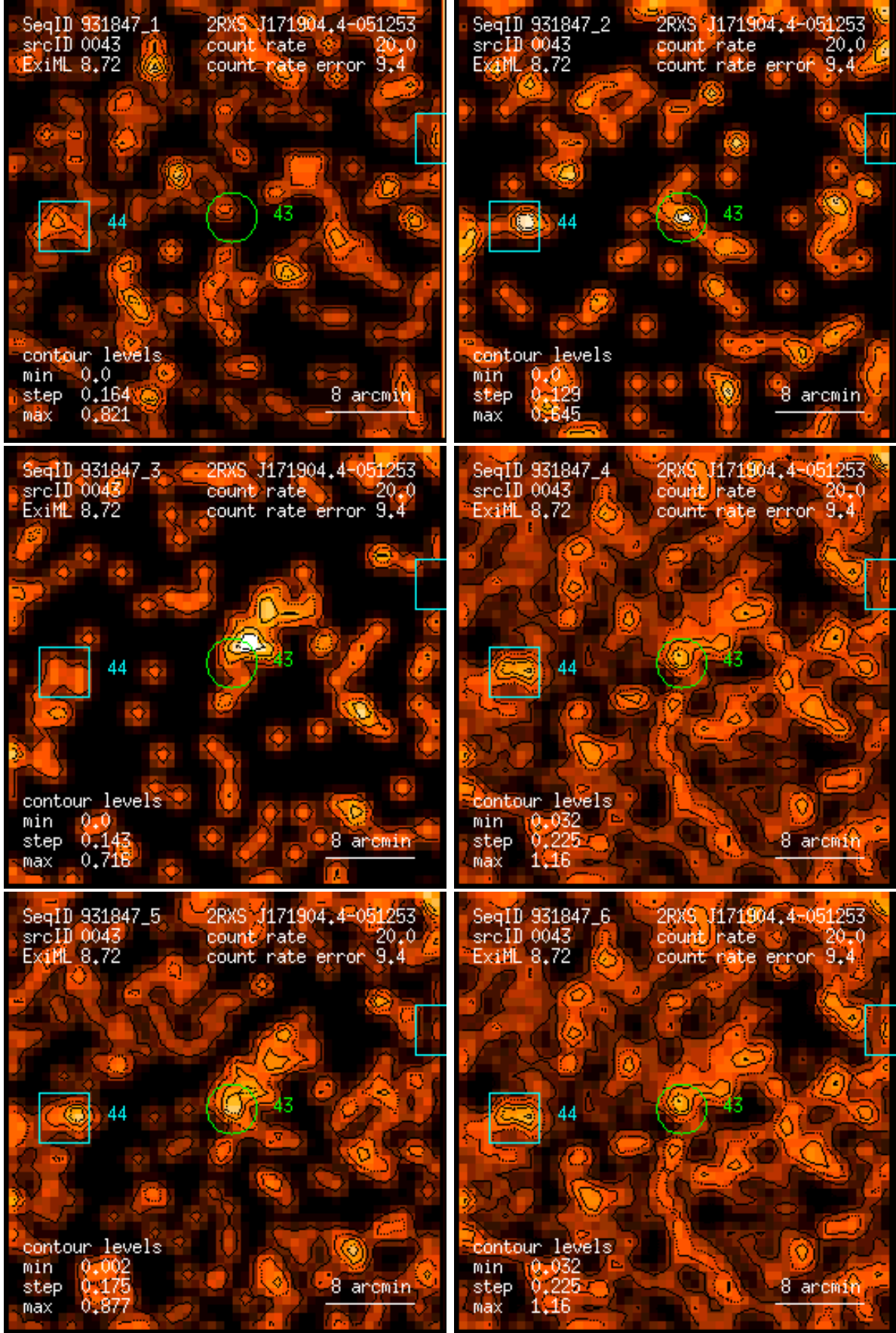
Figure 43: RASS 931847: detection 0043: band rate images, Gaussian filter: (1) PSPC channels 11 – 41, (2) 52 – 90, (3) 91 – 201, (4) 11 – 235, (5) 52 – 201, (6) 11 – 201. Broad band rates in counts/ks. Band rate contour levels in counts/ks/arcmin 2 .
