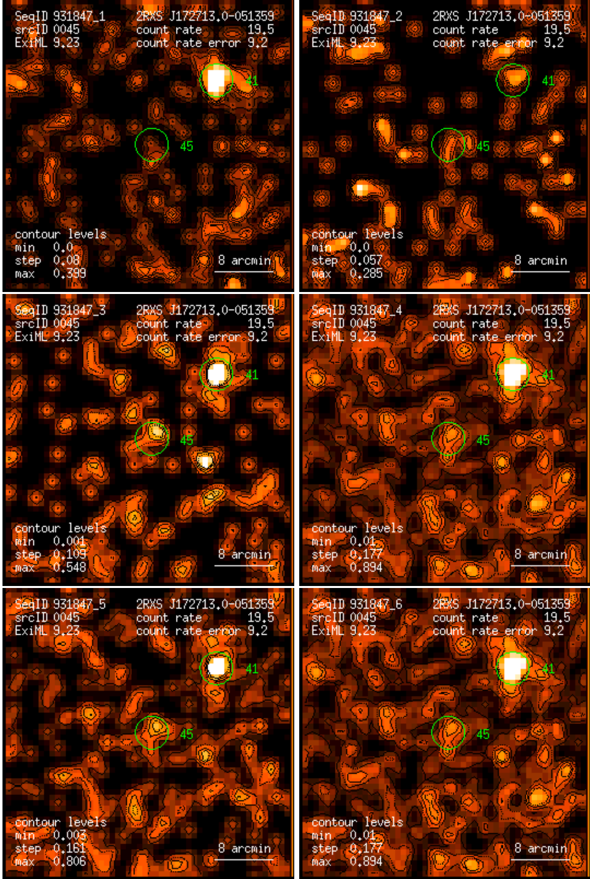
Figure 45: RASS 931847: detection 0045: band rate images, Gaussian filter: (1) PSPC channels 11 – 41, (2) 52 – 90, (3) 91 – 201, (4) 11 – 235, (5) 52 – 201, (6) 11 – 201. Broad band rates in counts/ks. Band rate contour levels in counts/ks/arcmin 2 .
