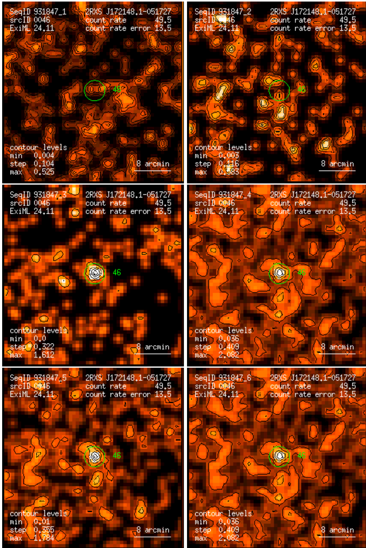
Figure 46: RASS 931847: detection 0046: band rate images, Gaussian filter: (1) PSPC channels 11 – 41, (2) 52 – 90, (3) 91 – 201, (4) 11 – 235, (5) 52 – 201, (6) 11 – 201. Broad band rates in counts/ks. Band rate contour levels in counts/ks/arcmin 2 .
