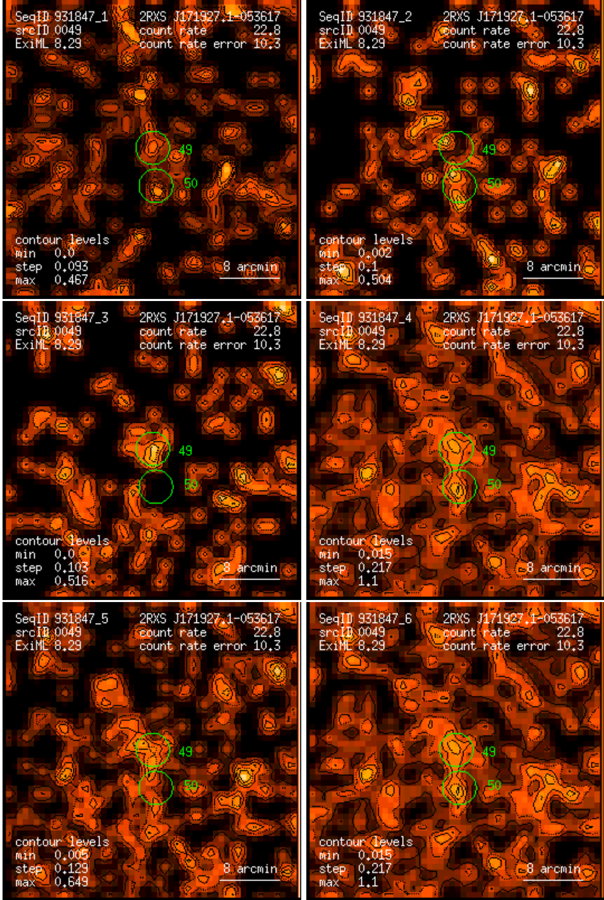
Figure 49: RASS 931847: detection 0049: band rate images, Gaussian filter: (1) PSPC channels 11 – 41, (2) 52 – 90, (3) 91 – 201, (4) 11 – 235, (5) 52 – 201, (6) 11 – 201. Broad band rates in counts/ks. Band rate contour levels in counts/ks/arcmin 2 .
